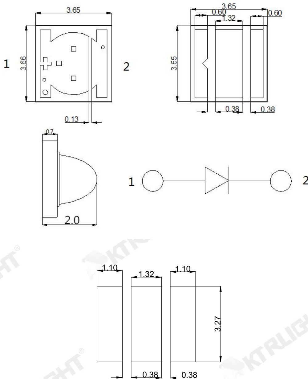
推荐焊盘式样(Recommended Soldering Patter)
