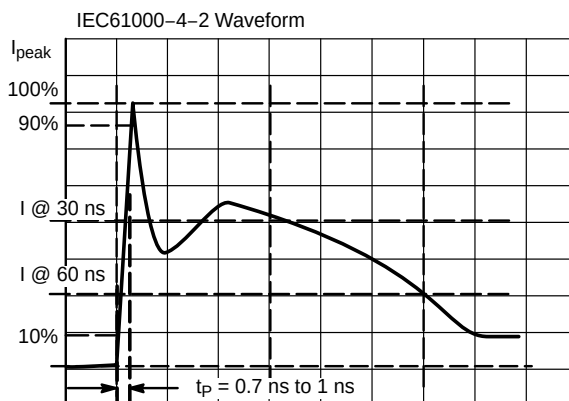
Figure 3. IEC61000-4-2 Spec
