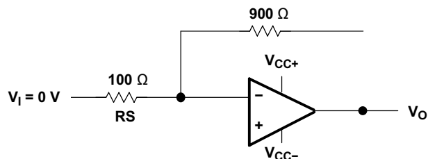
Figure 8. Noise-Test Circuit
