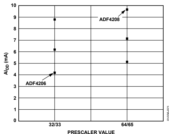
Figure 21. ADF4206/ADF4208 A_{LD} vs. Prescaler Value (RF1)
