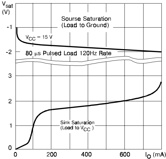
Figure 7. Output Saturation Voltage vs. Load Current T_A = 25^{\circ}C
