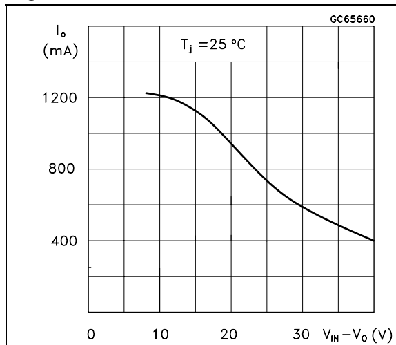
Figure 4. Current limit
