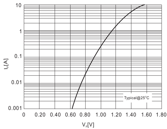
Fig.1-TYPICAL FORWARD CHARACTERISTICS
