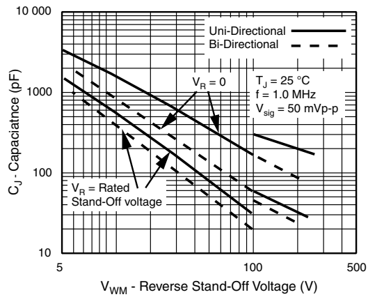
Figure 6. Capacitance
