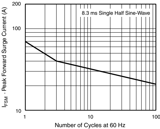
Figure 4. Maximum Non-Repetitive Forward Surge Current Uni-Directional Only
