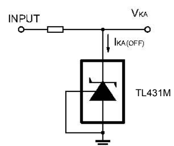
Test Circuit For I_{KA}(\text{OFF})
