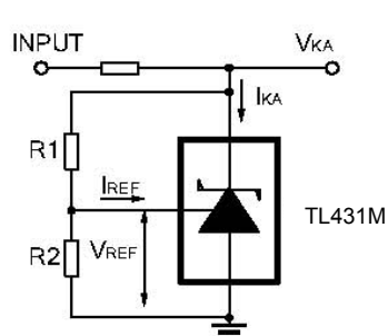
V_{KA}=V_{REF}(1+R1/R2)+I_{REF}R1 Test Circuit for V_{KA} \geq V_{REF}
