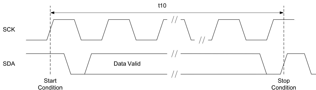
Figure 27. Master I2C for EEPROM Auto-load Timing
