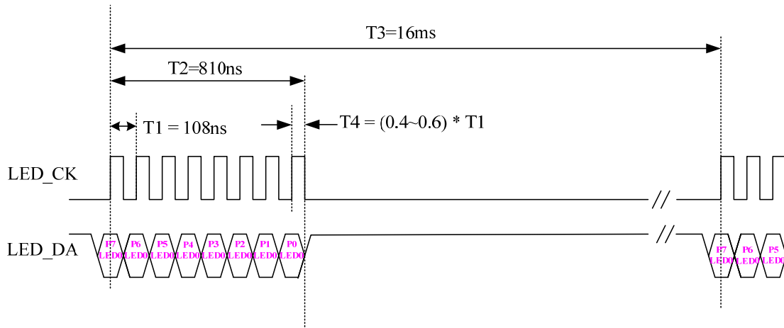
Figure 15. RTL8370N-VB serial led mode shift sequence (per-port one single-color LED)
