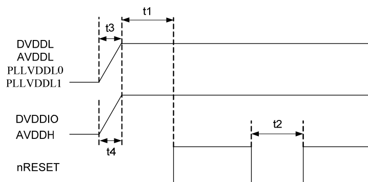
Figure 31. Power and Reset Characteristics
