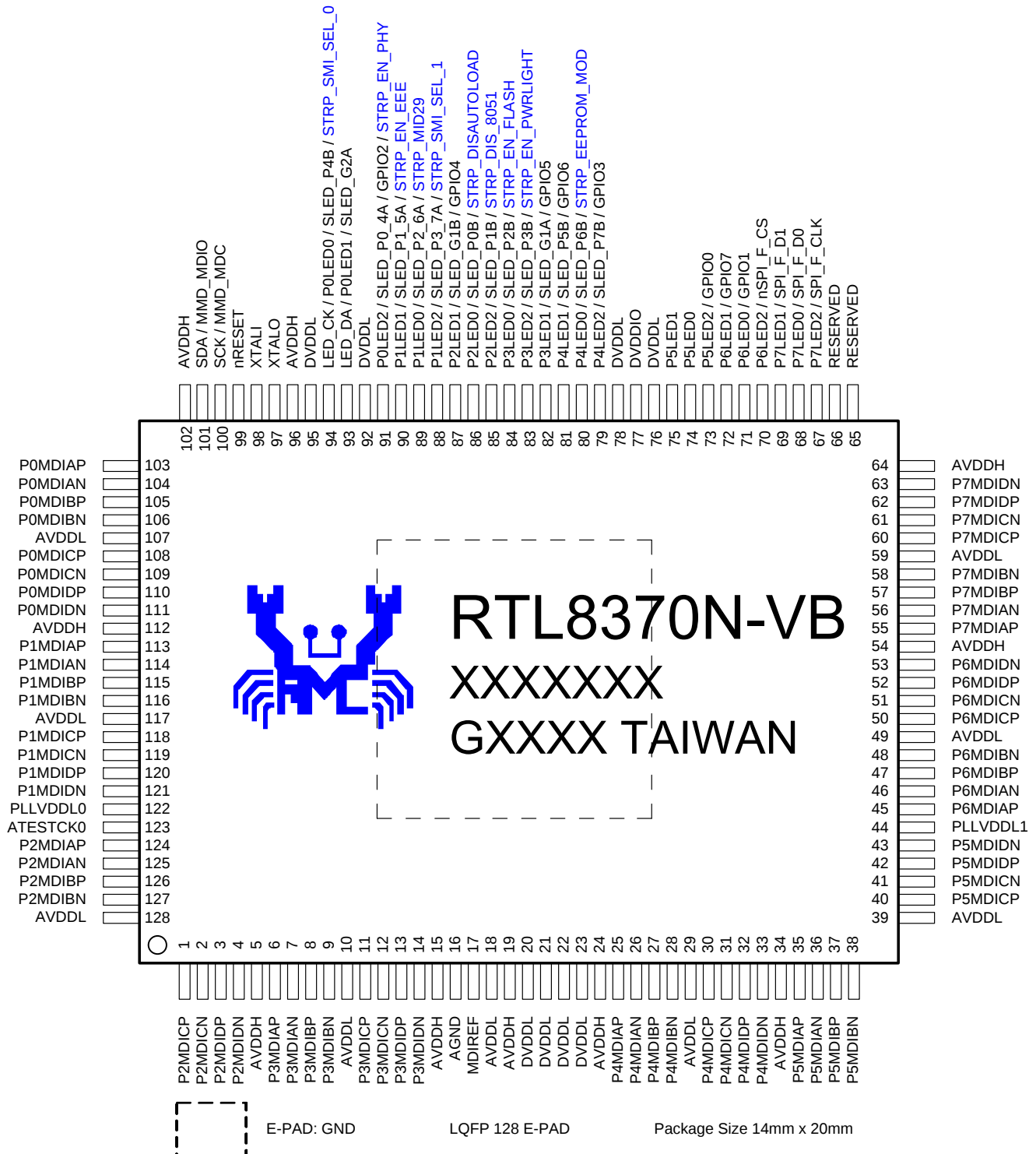
Figure 3. RTL8370N-VB Pin Assignments (LQFP-128-EPAD)
