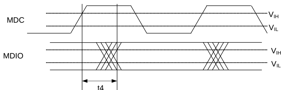
Figure 30. MDIO Sourced by Slave (RTL8370N-VB)
