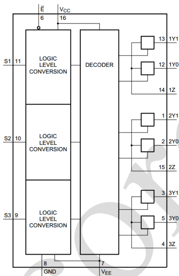
Figure 4. Functional diagram
