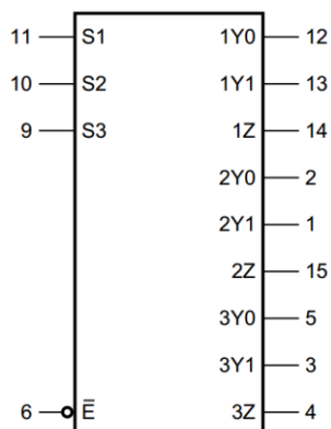
Figure 1. Logic symbol
