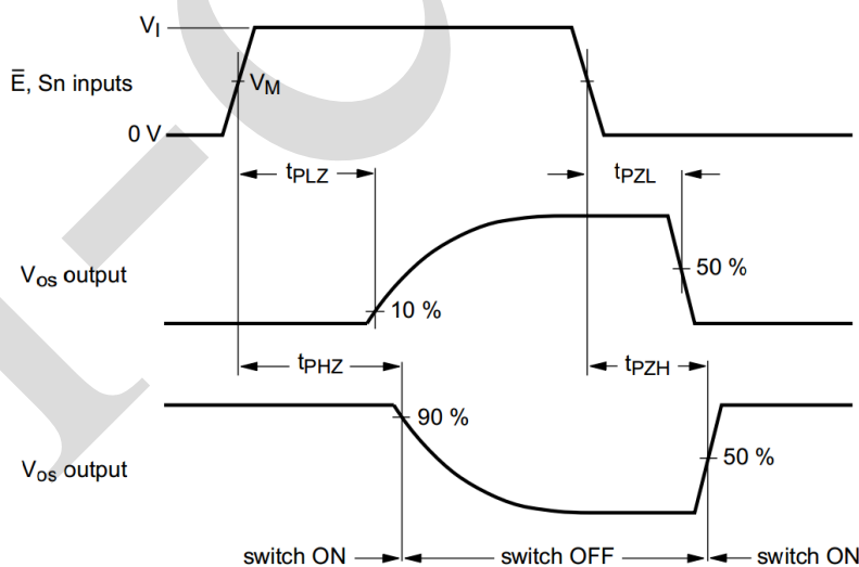
Figure 9. Input ( V_{is} ) to output ( V_{os} ) propagation delays
