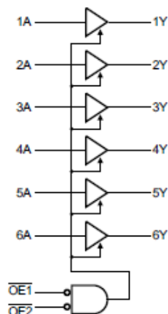
Figure 1. Logic symbol
