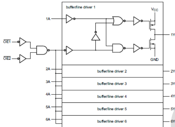
Figure 4. Logic diagram
