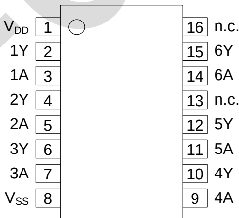
Figure 4. Pin configuration
