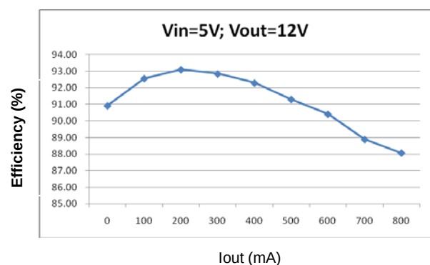
Figure 2. Efficiency Curve
