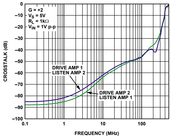
Figure 39. ADA4851-2, RTI Crosstalk vs. Frequency
