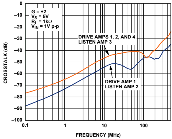
Figure 38. ADA4851-4, RTI Crosstalk vs. Frequency
