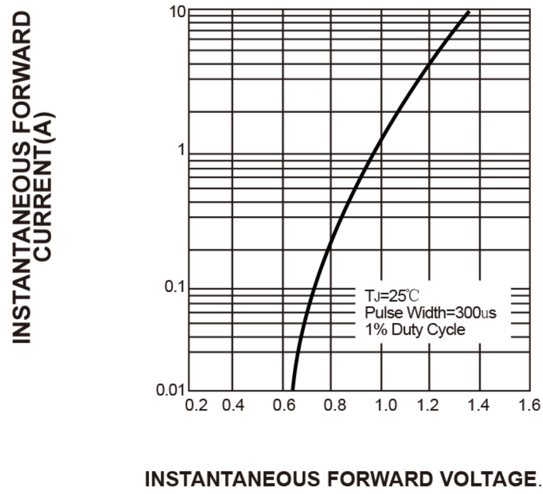
FIG. 3-TYPICAL FORWARD VOLTAGE CHARACTERISTICS PER LEG
