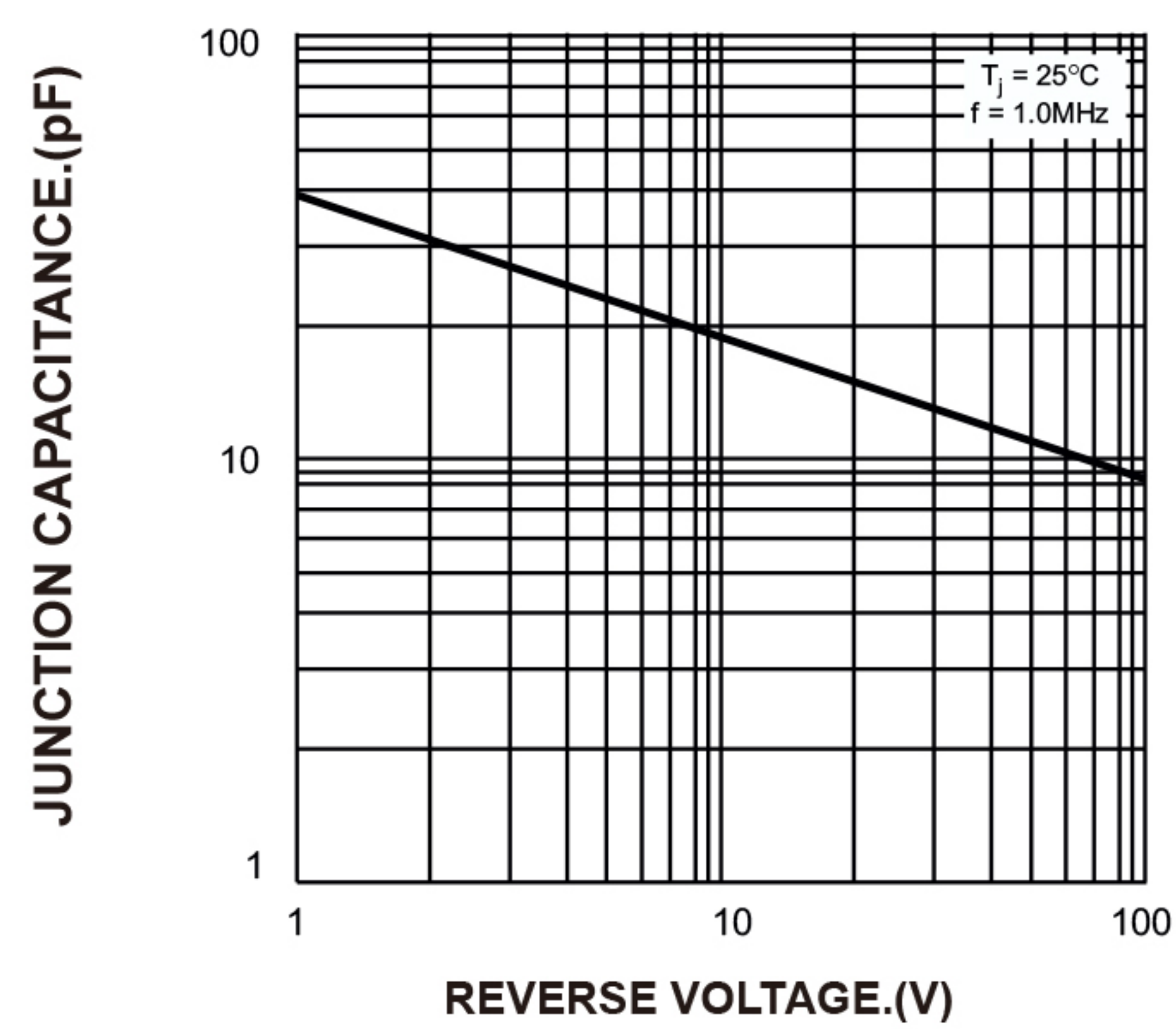
FIG. 5-TYPICAL JUNCTION CAPACITANCE PER LEG
