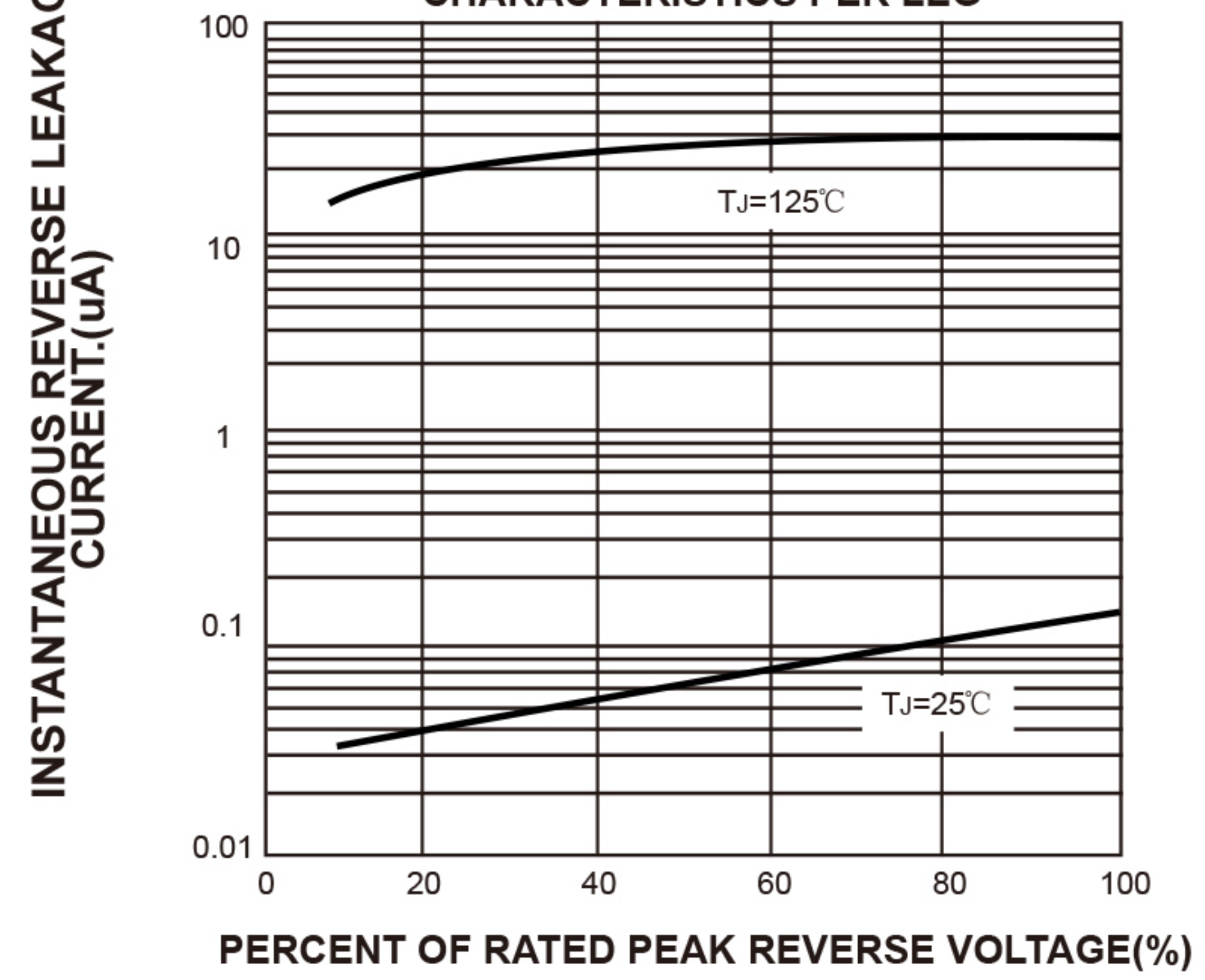
FIG. 4-TYPICAL REVERSE LEAKAGE CHARACTERISTICS PER LEG
