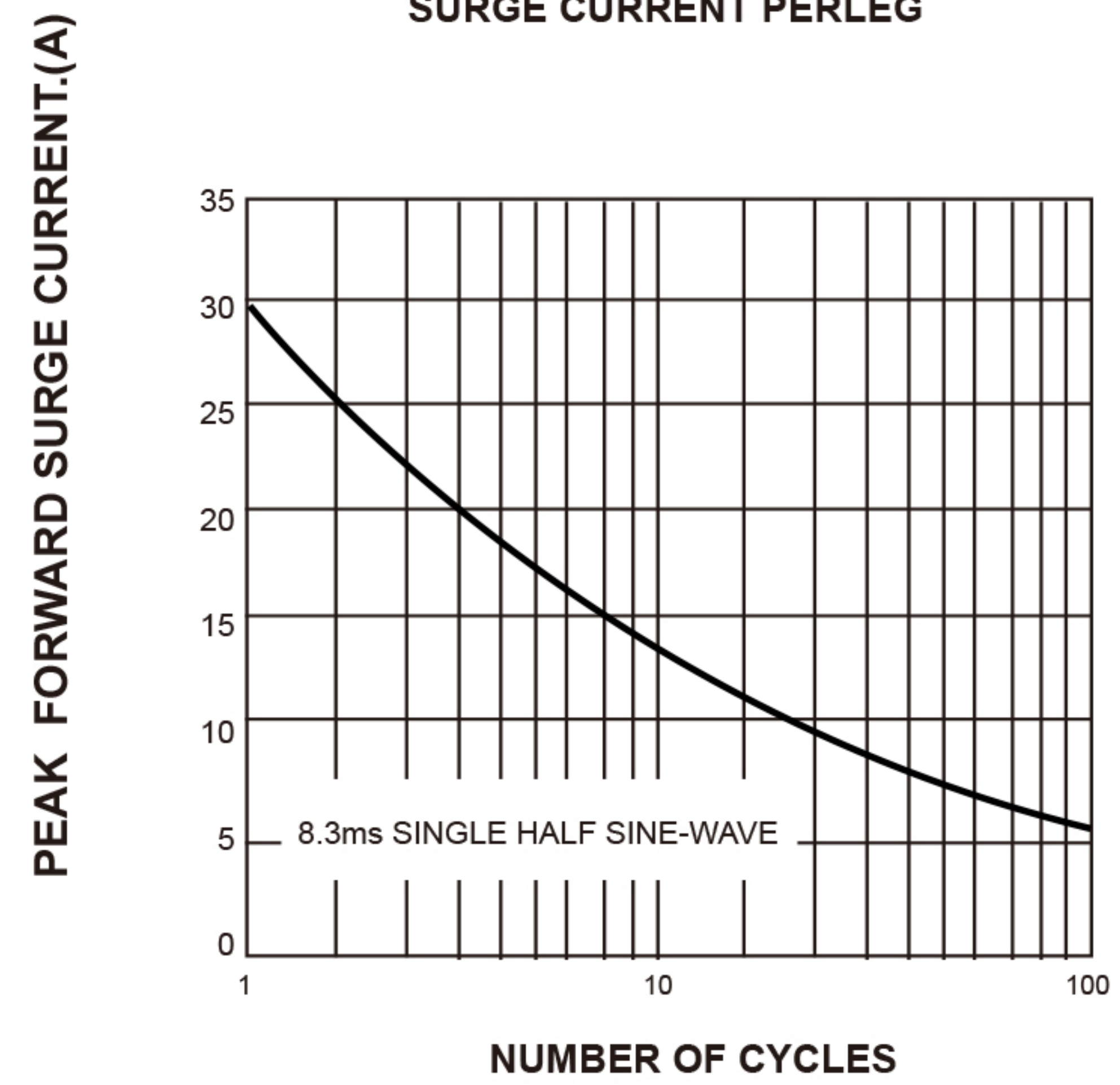
FIG. 2-MAXIMUM NON-REPETITIVE PEAK FORWARD SURGE CURRENT PERLEG
