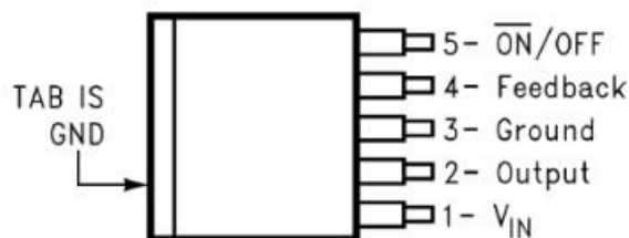
TO-263 (S) Top View
