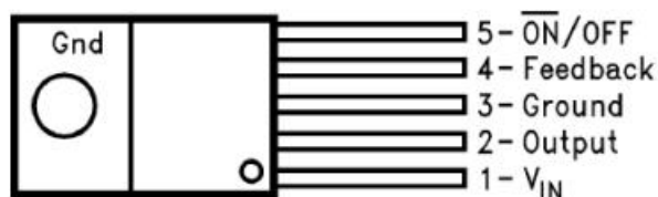
TO-220 (T) Top View
