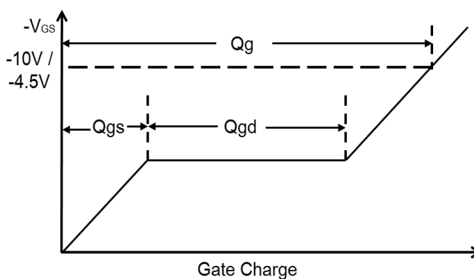
Fig.11 Gate Charge Waveform
