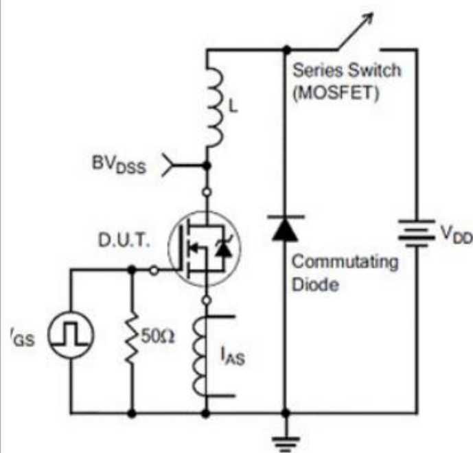
Figure 18 Unclamped Inductive Switching Test Circuit
