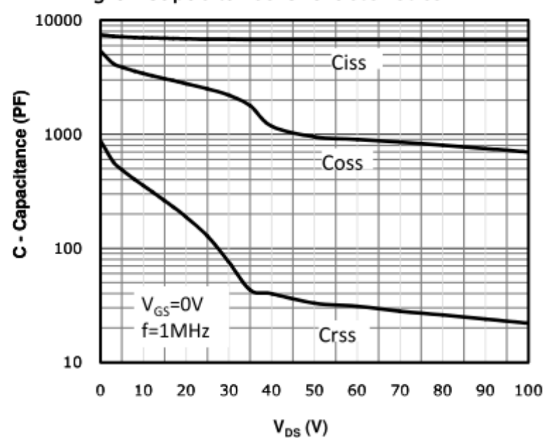
Fig 6: Capacitance Characteristics
