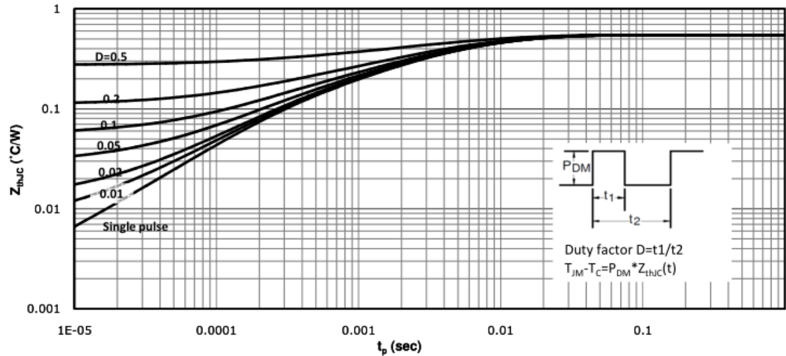
Fig 12: Max. Transient Thermal Impedance
