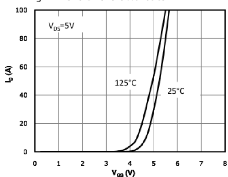
Fig 2: Transfer Characteristics
