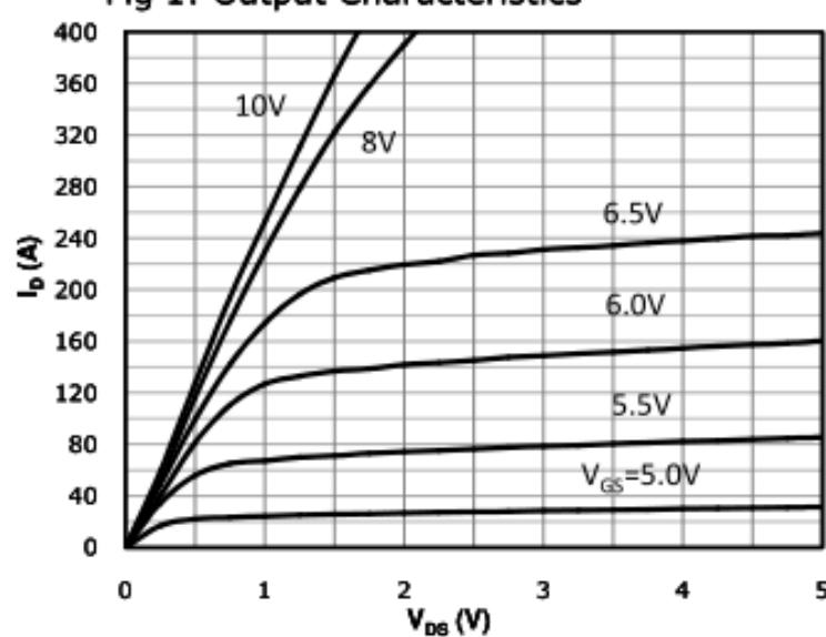
Fig 1: Output Characteristics
