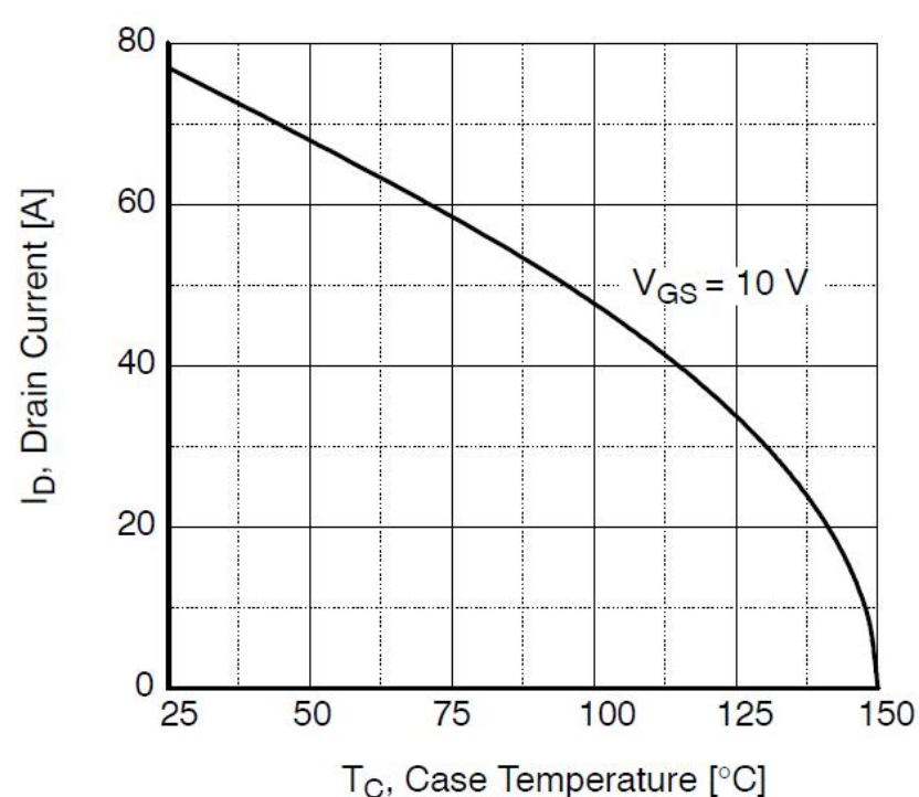
Figure 10. Maximum Drain Current vs. Case Temperature
