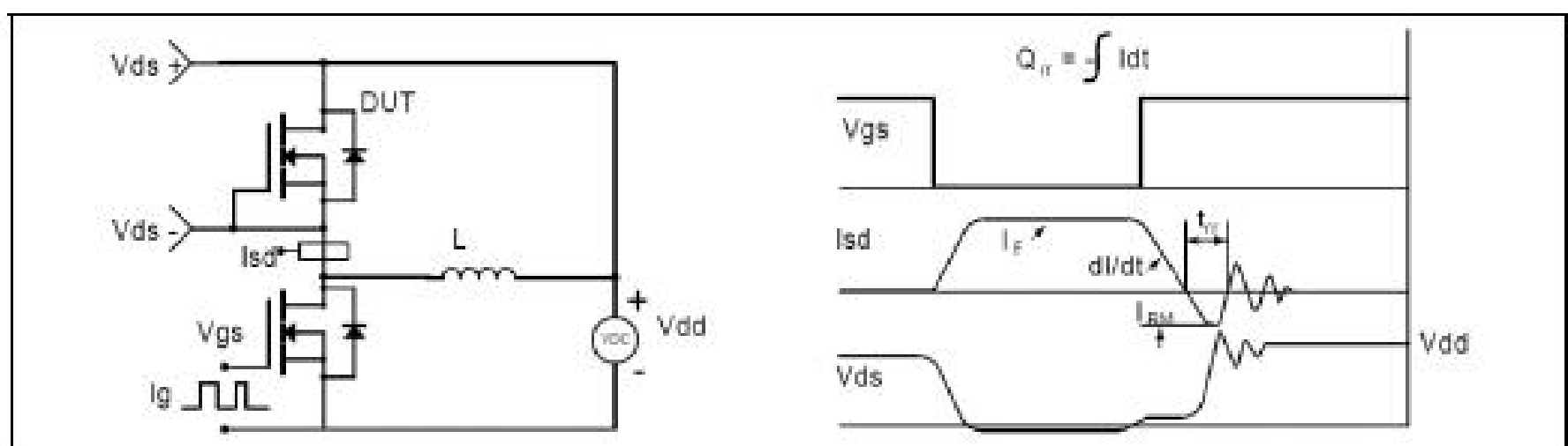
Figure 4. Diode reverse recovery test circuit & waveforms
