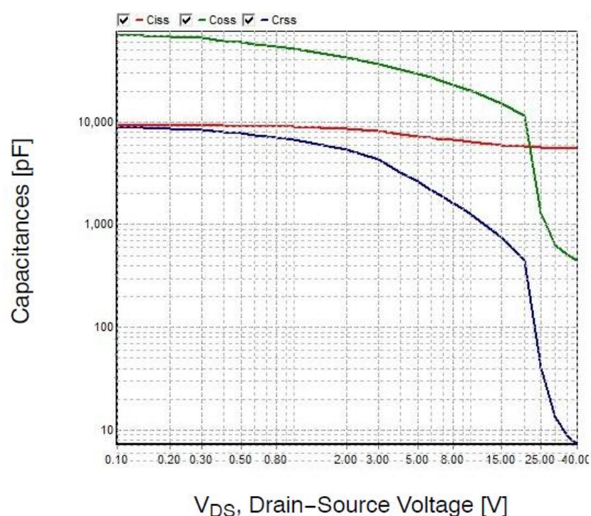
Figure 5. Capacitance Characteristics
