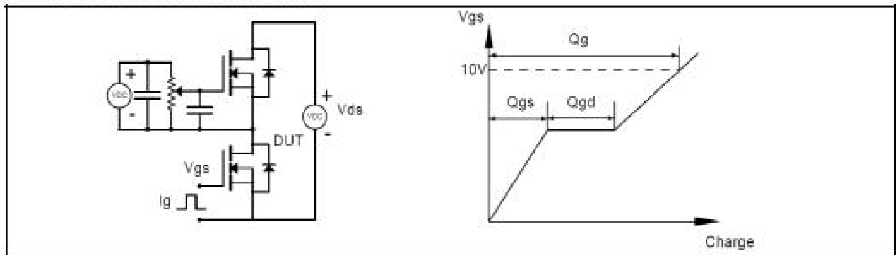
Figure 1. Gate charge test circuit & waveform
