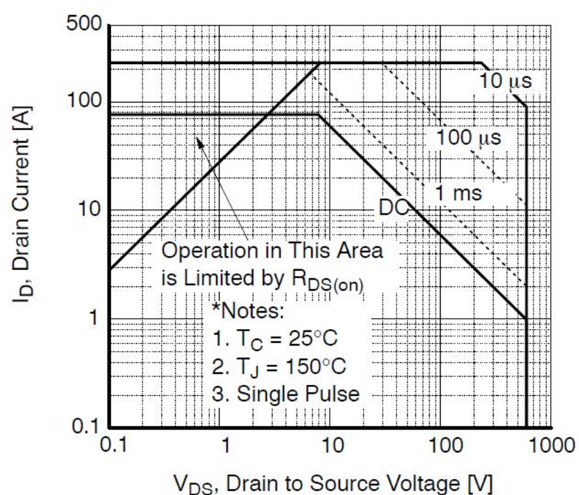
Figure 9. Maximum Safe Operation Area
