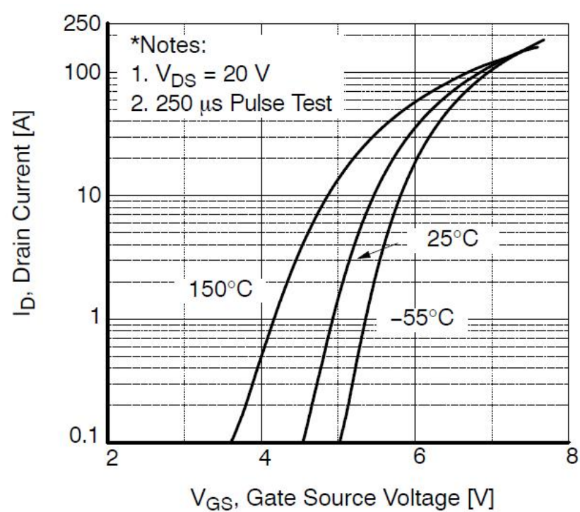
Figure 2. Transfer Characteristics
