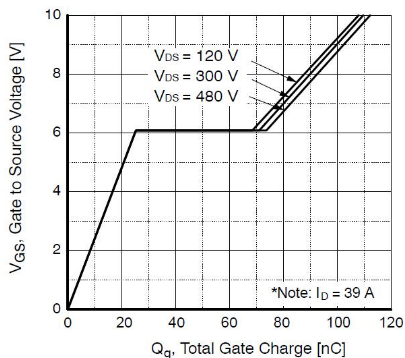
Figure 6. Gate Charge Characteristics
