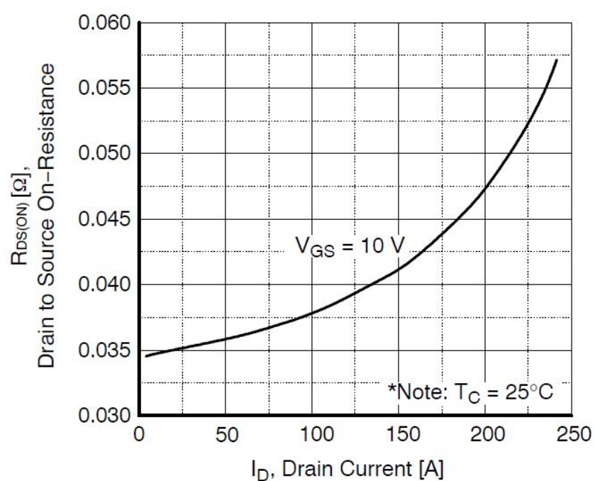
Figure 3. On-Resistance Variation vs. Drain Current
