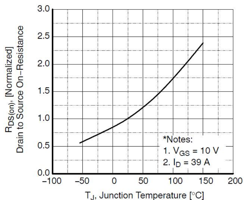
Figure 8. On-Resistance Variation vs. Temperature
