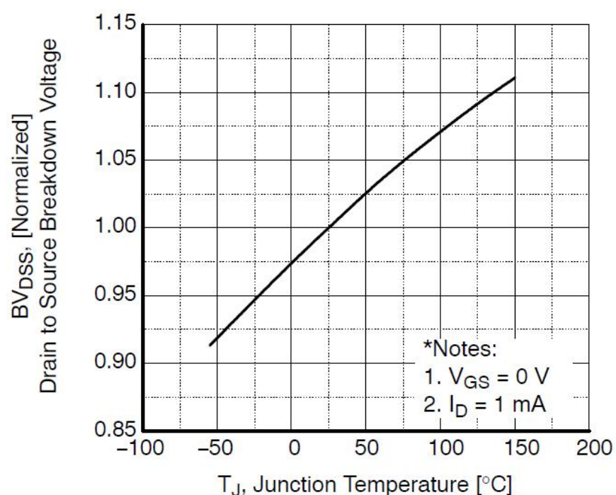
Figure 7. Breakdown Voltage Variation vs. Temperature
