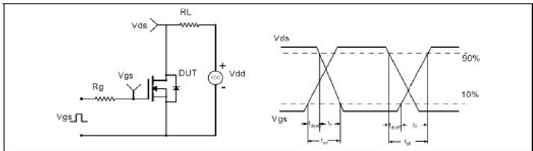
Figure 2. Switching time test circuit & waveforms
