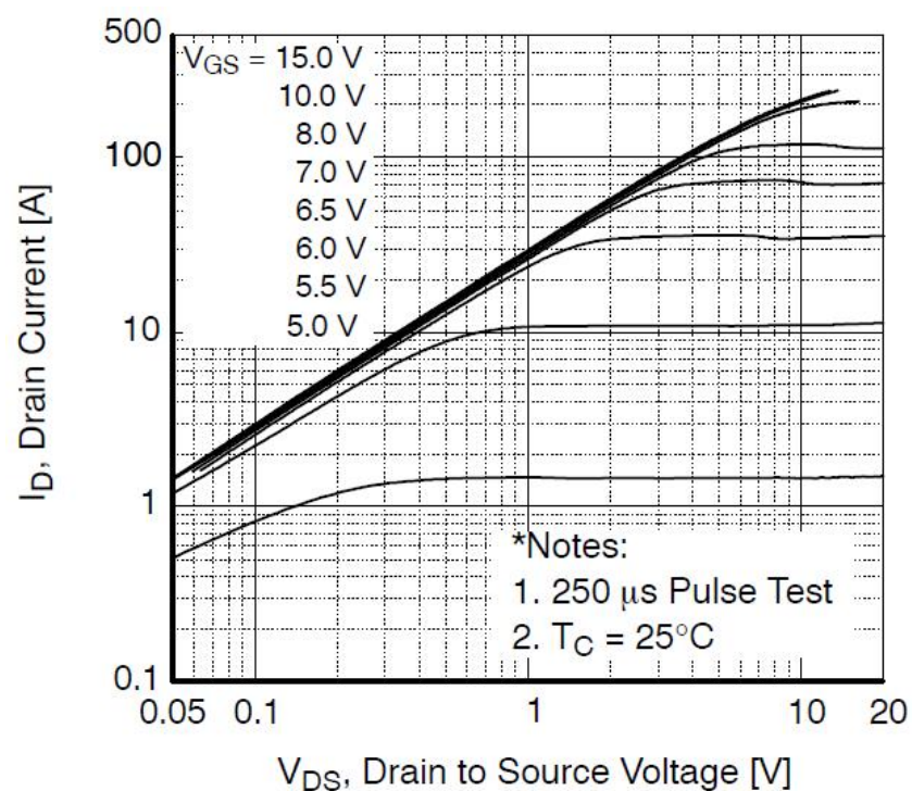
Figure 1. On-Region Characteristics
