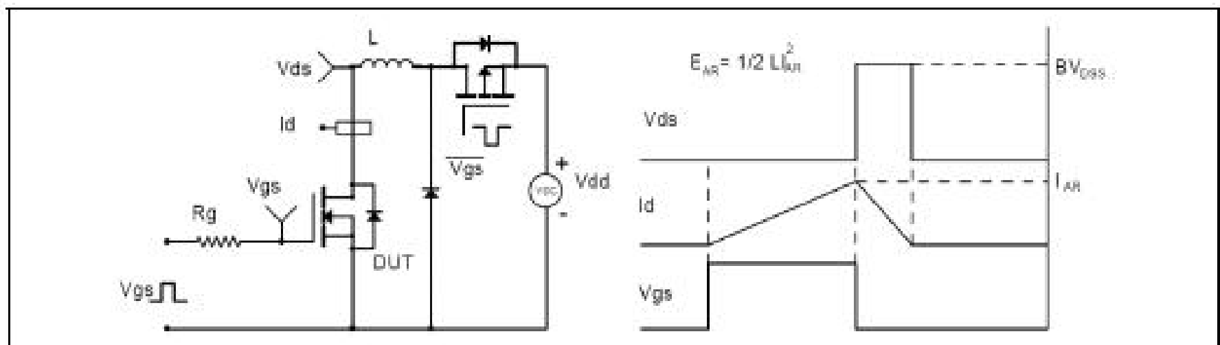
Figure 3. Unclamped inductive switching (UIS) test circuit & waveforms
