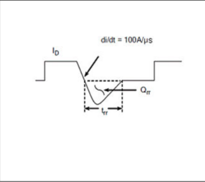
Figure 17 Diode Reverse Recovery Waveform
