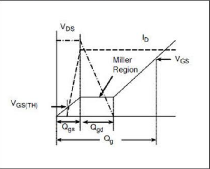
Figure 13 Gate Charge Waveforms
