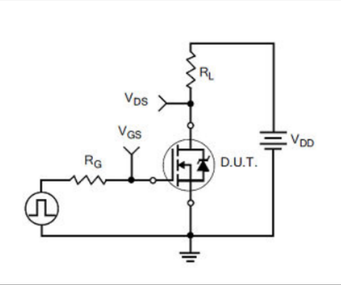
Figure 14 Resistive Switching Test Circuit
