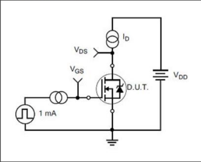
Figure 12 Gate Charge Test Circuit
