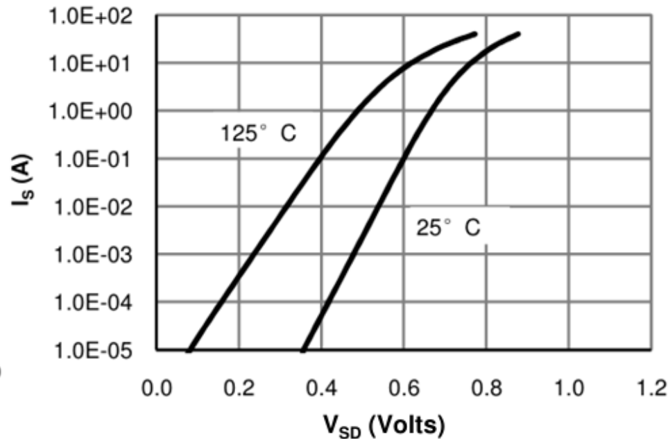
Figure 6: Body-Diode Characteristics
