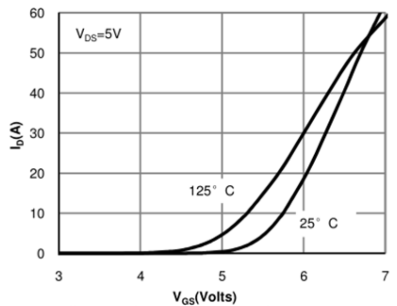
Figure 2: Transfer Characteristics
