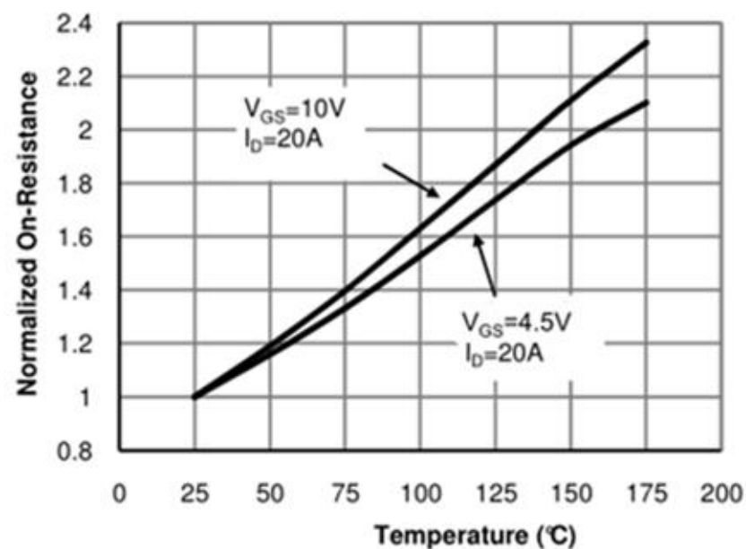
Figure 4: On-Resistance vs. Junction Temperature
