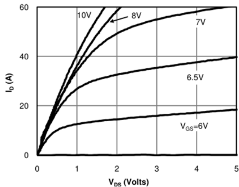
Fig 1: On-Region Characteristics
