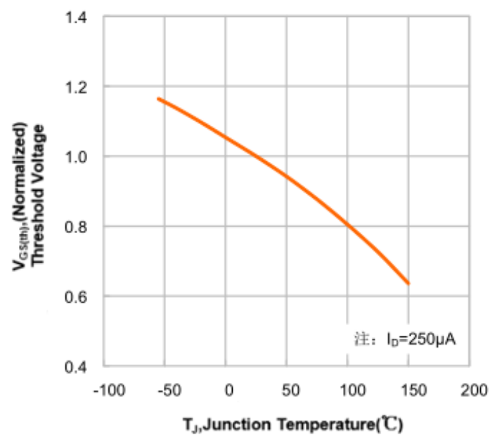
Typical Theshold Voltage vs Junction Temperature
