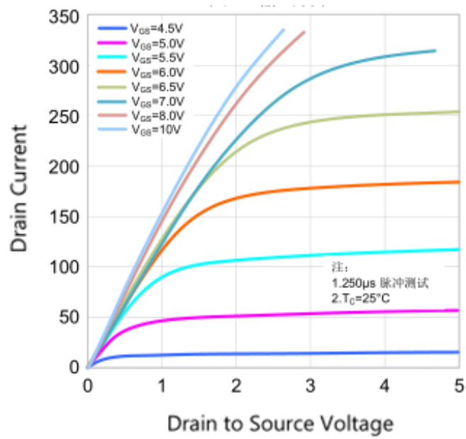
Output Characteristics
