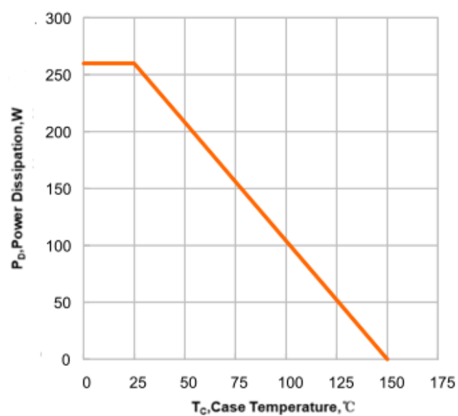
Maximum Power dissipation vs Case Temperature
