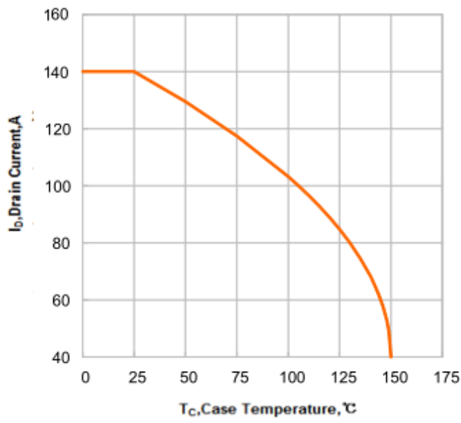
Maximum Continuous Drain Current vs Case Temperature
