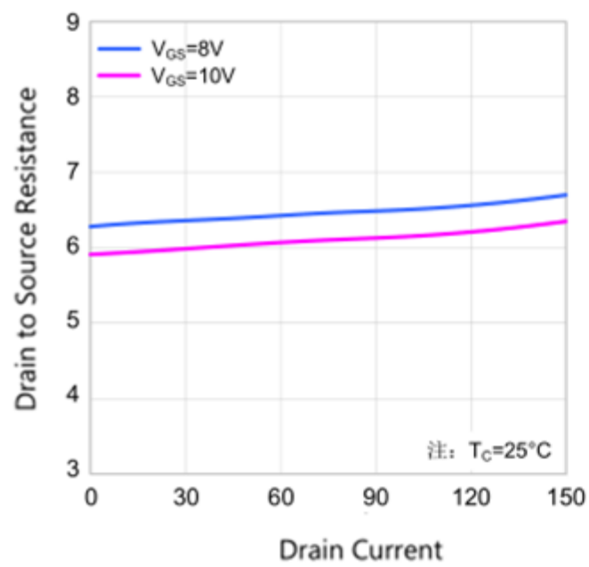
Drain to Source Resistance vs. Drain Current
