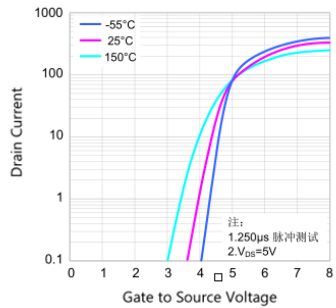
Transfer Characteristics
