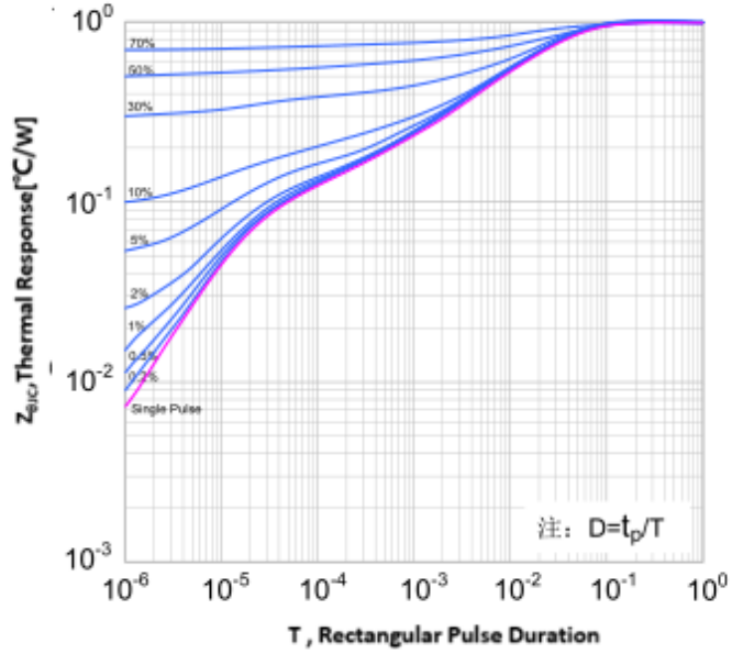
Maximum Effective Thermal Impedance , Junction to Case
