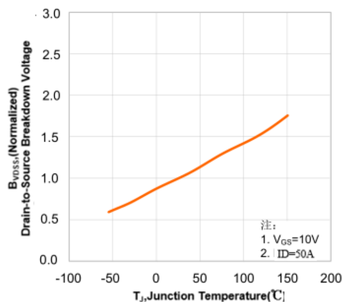
Typical Breakdown Voltage vs Junction Temperature
