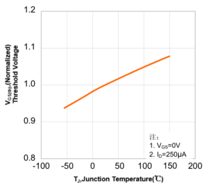
Typical Theshold Voltage vs Junction Temperature
