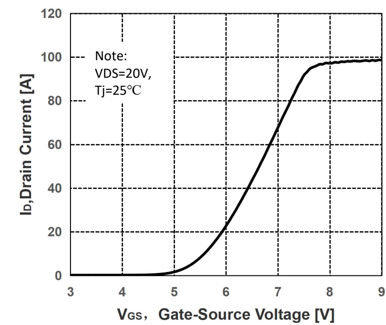
Figure 5. Typical Transfer Characteristics
