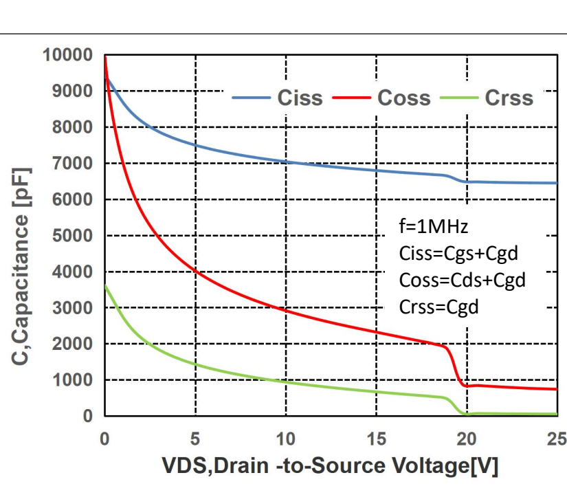
Figure 11. Capacitance Characteristics
