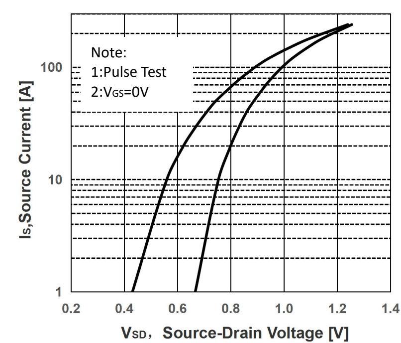
Figure 6. Source-Drain Diode Forward Characteristics
