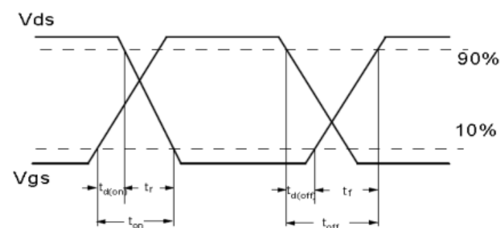
Resistive Switching Test Circuit & Waveforms
