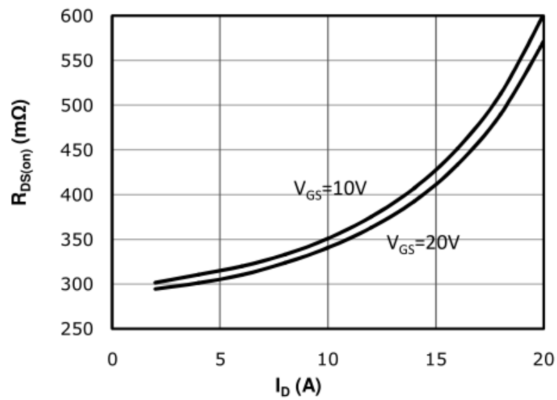
Fig 5: R_{DS(on)} Vs I_{DS} Characteristics ( T_c=25^\circ\text{C} )
