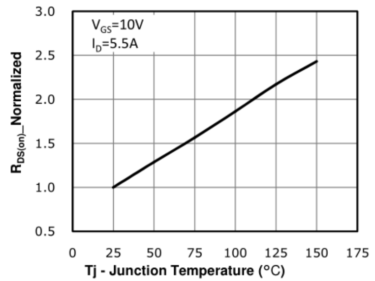
Fig 6: R_{DS(on)} vs. Temperature
