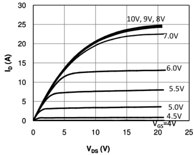
Fig 1. Output Characteristics ( T_J=25^\circ\text{C} )
