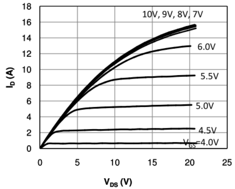
Fig 2. Output Characteristics ( T_J=150^\circ\text{C} )
