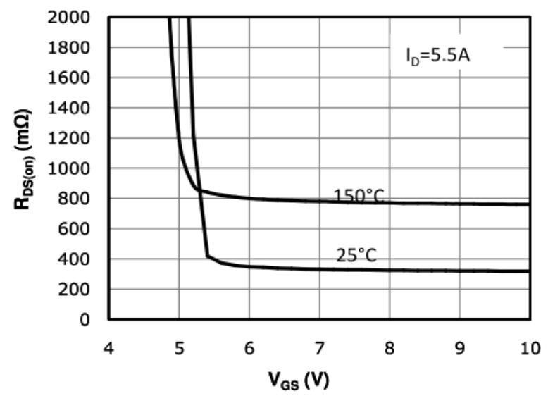
Fig 8: Rds(on) vs Gate Voltage
