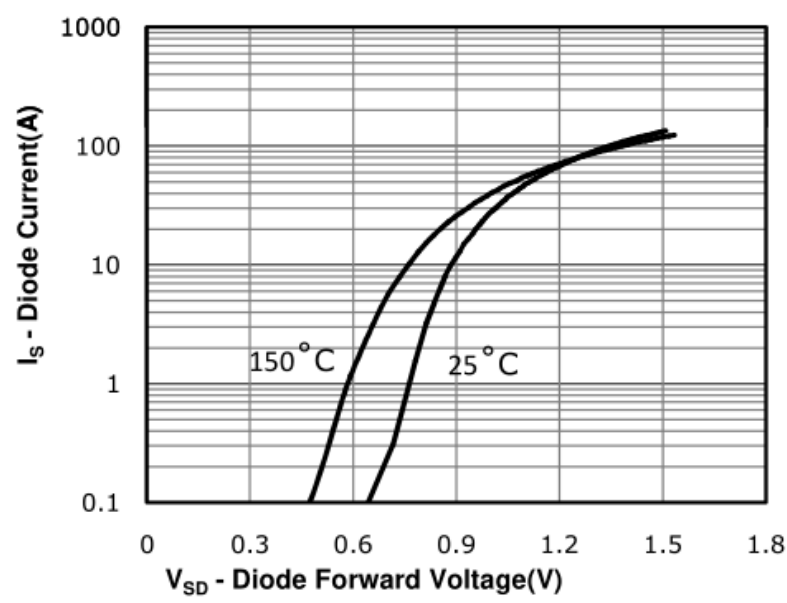
Fig 9: Body-diode Forward Characteristics
