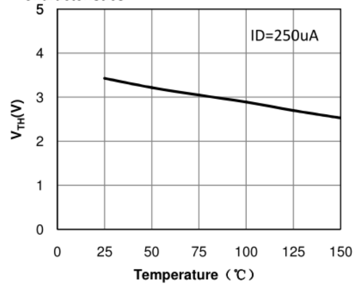
Fig 4: V_{TH} Vs T_J Temperature Characteristics
