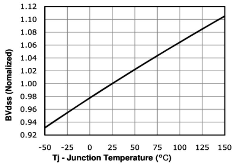
Fig 7: BVDSS vs. Temperature
