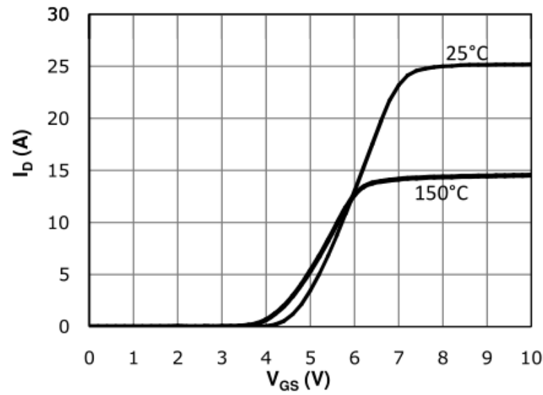
Fig 3: Transfer Characteristics
