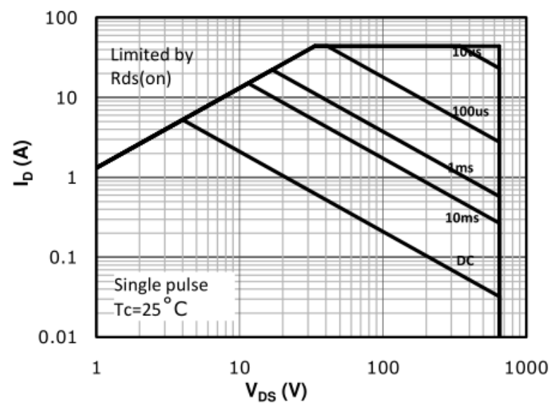
Fig 12: Safe Operating Area
