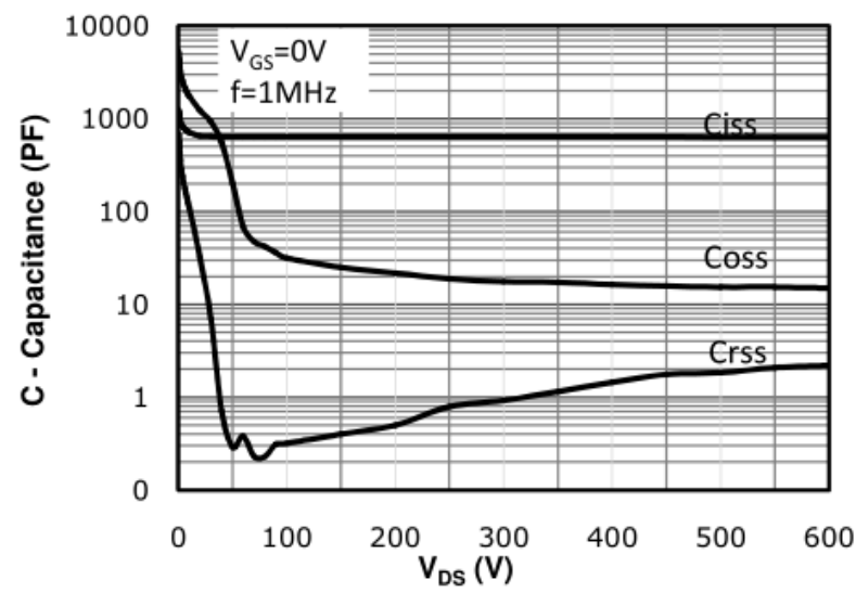
Fig 11: Capacitance Characteristics
