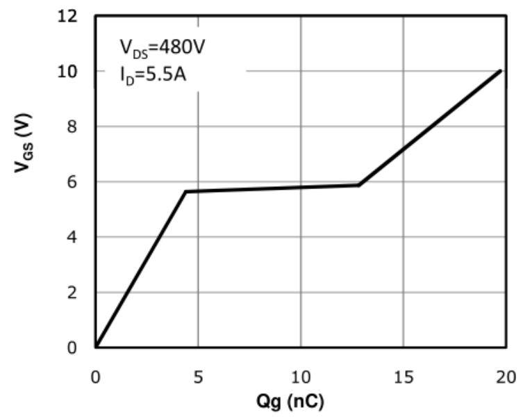
Fig 10: Gate Charge Characteristics
