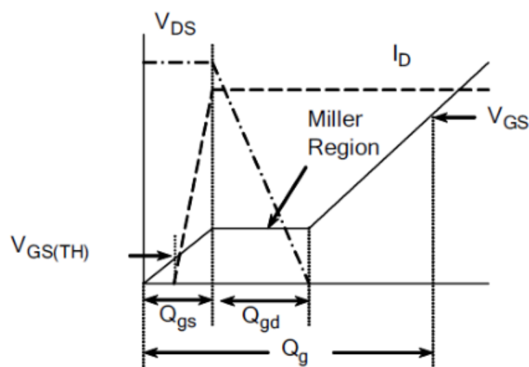
Figure 15. Gate Charge Waveforms
