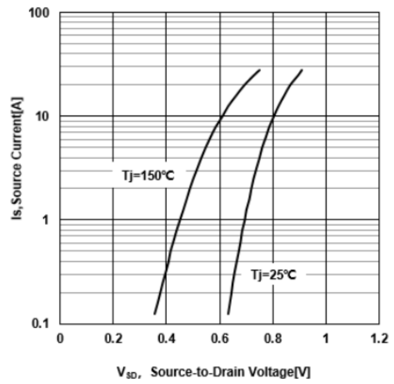
Figure 7 Typical Body Diode Transfer Characteristics
