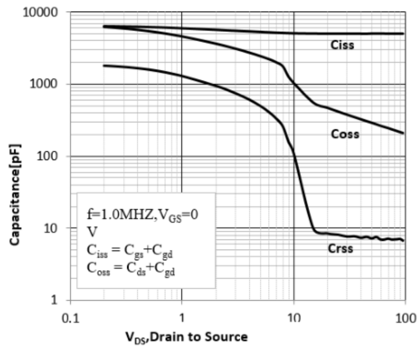
Figure 12 Typical Capacitance vs Drain to Source Voltage
