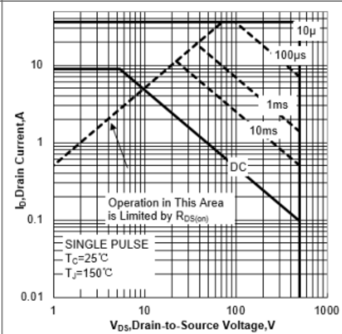
Figure 1b Safe Operating Area (FullPAK)
