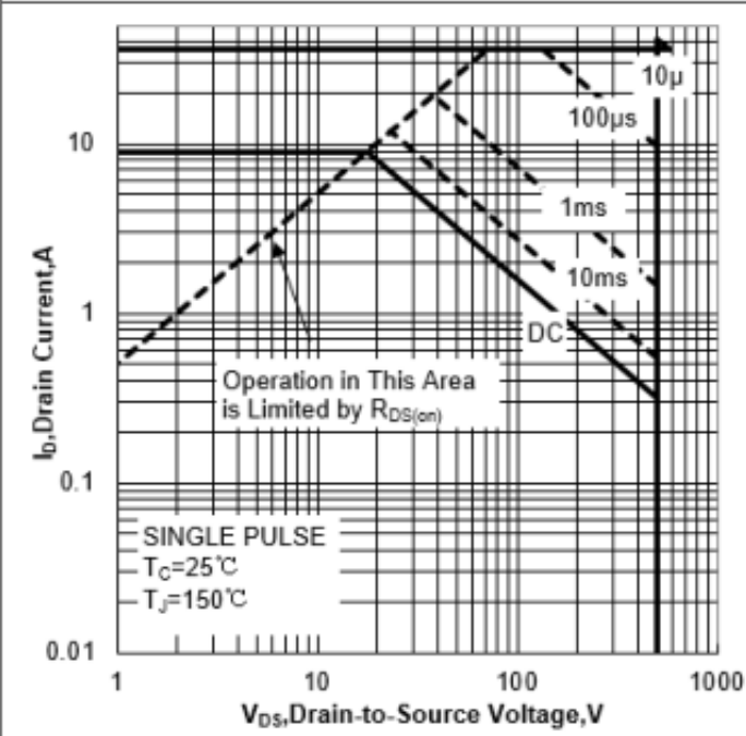
Figure 1a Safe Operating Area (No FullPAK)
