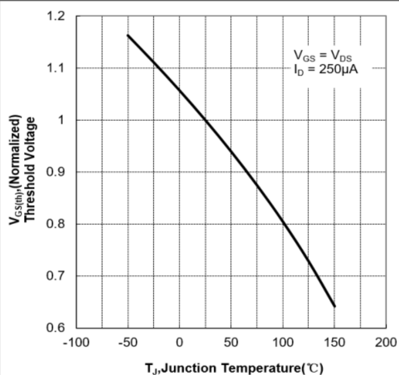
Figure 8 Typical Threshold Voltage vs Junction Temperature
