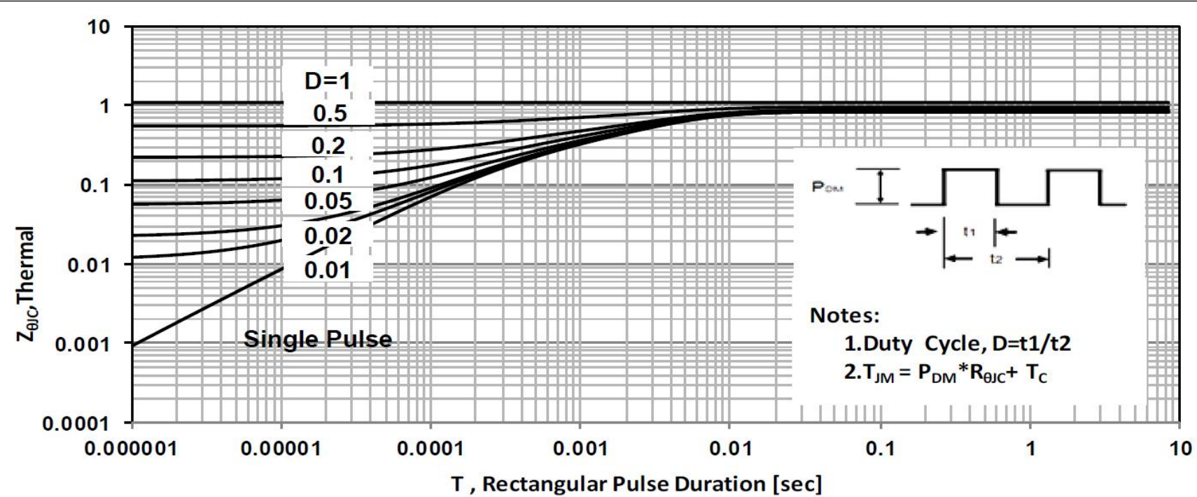
Figure 13. Transient Thermal Impedance
