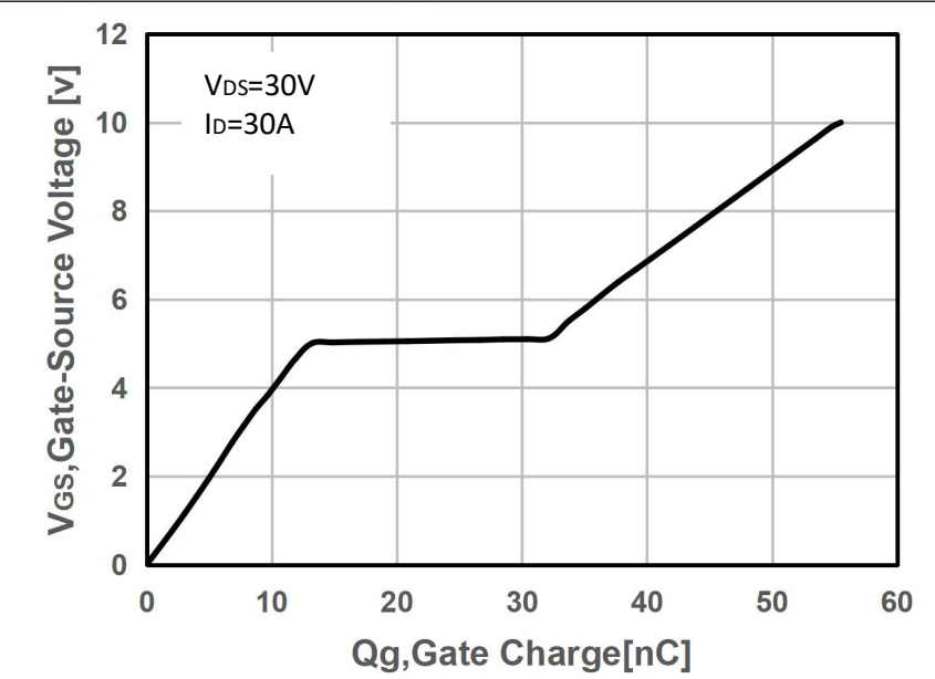
Figure 12. Typical Gate Charge vs Gate-Source Voltage
