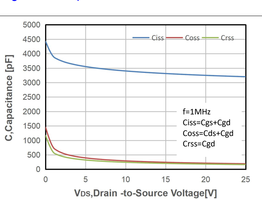
Figure 11. Capacitance Characteristics
