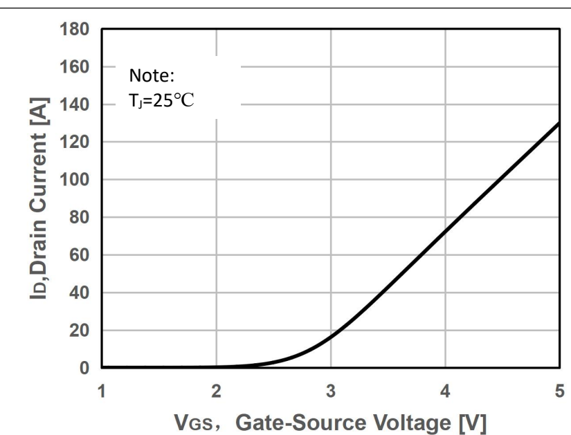
Figure 5. Typical Transfer Characteristics
