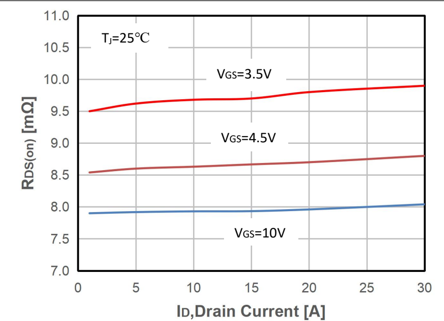
Figure 7. Drain-Source On-Resistance vs Drain Current
