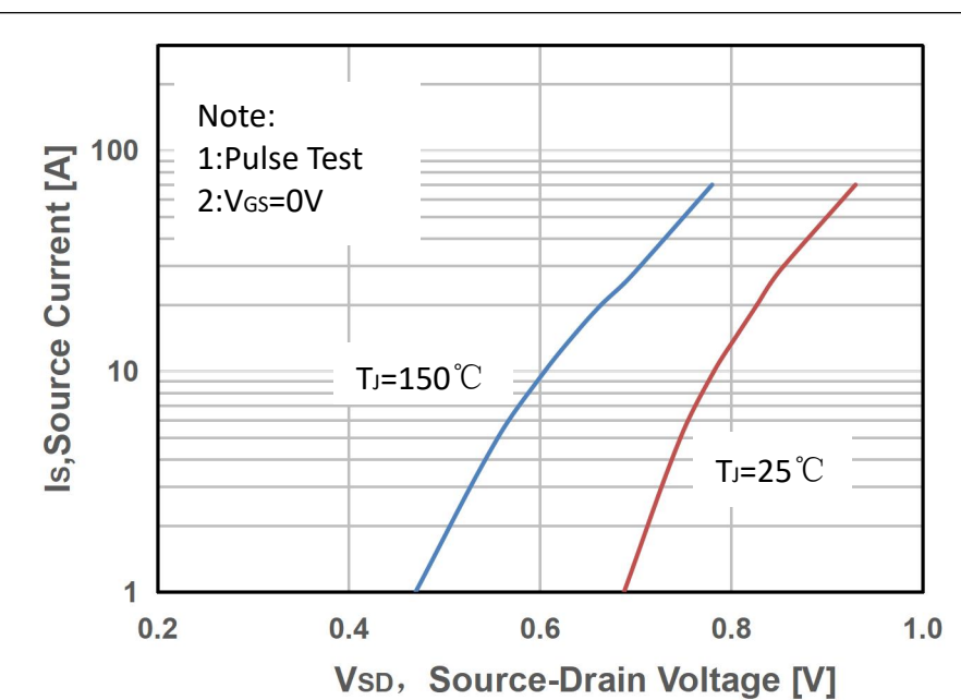
Figure 6. Source-Drain Diode Forward Characteristics
