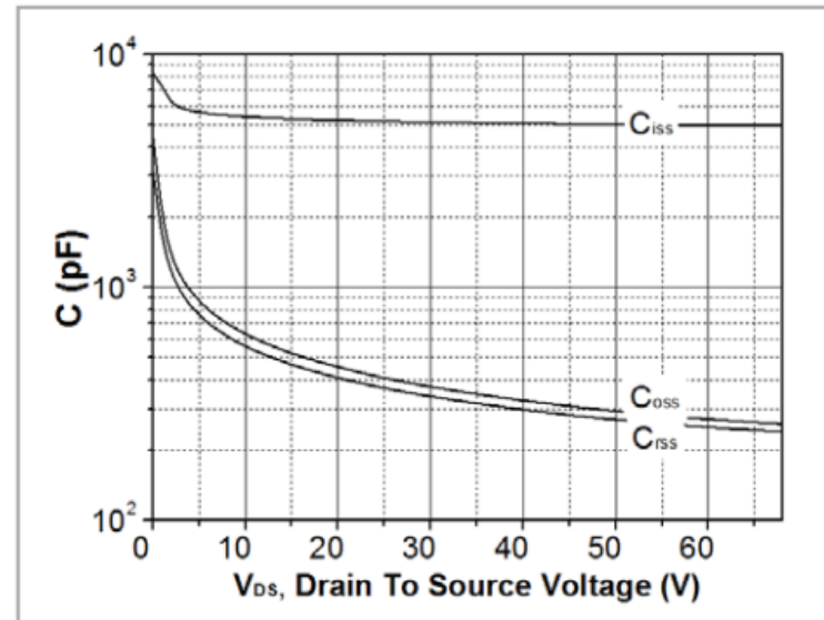
Fig. 8. Capacitance Characteristics
