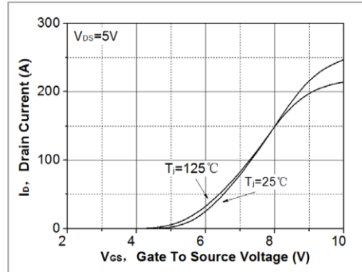
Fig. 2. Transfer Characteristics
