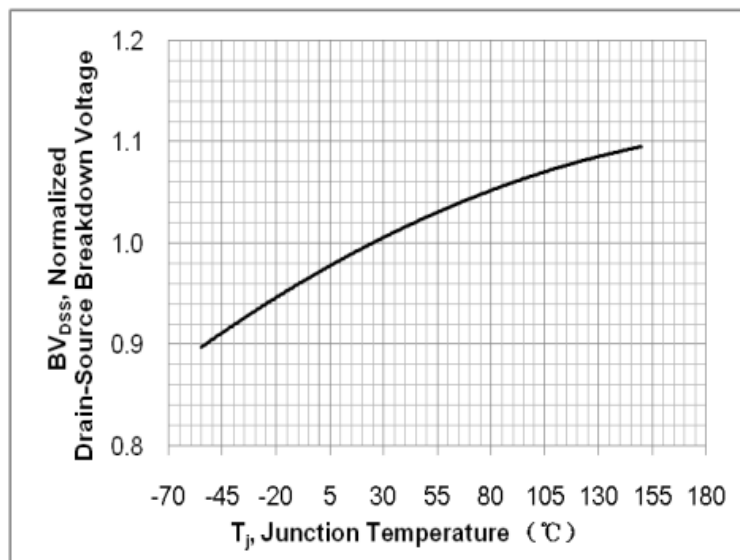
Fig 5. Breakdown voltage variation vs. junction temperature
