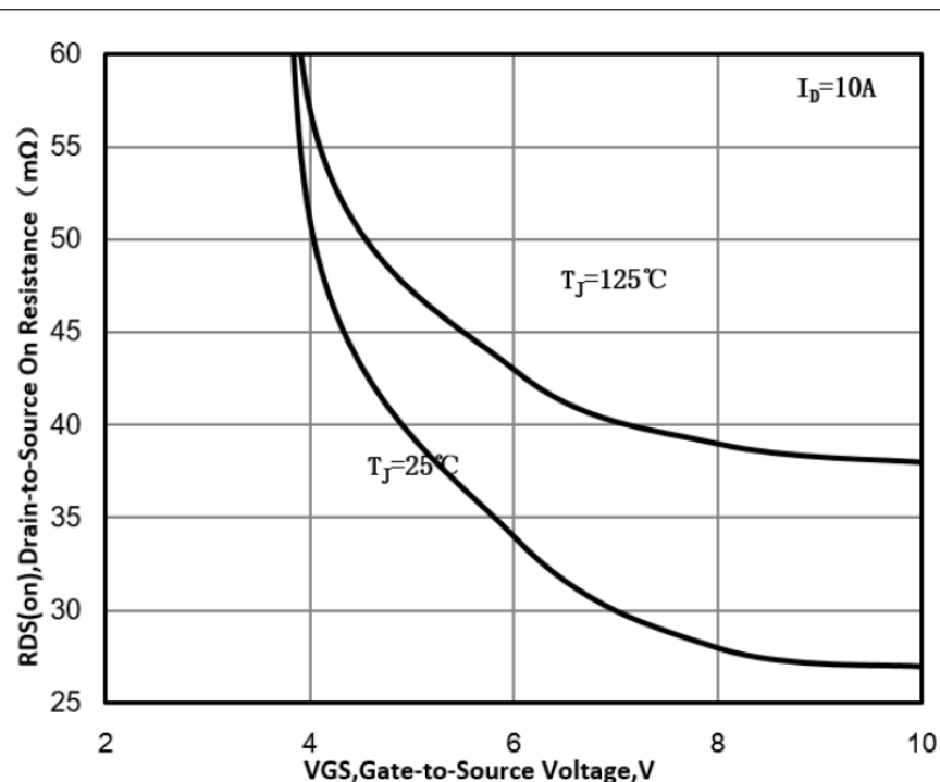
Figure 5 On-Resistance vs. V_{GS}
