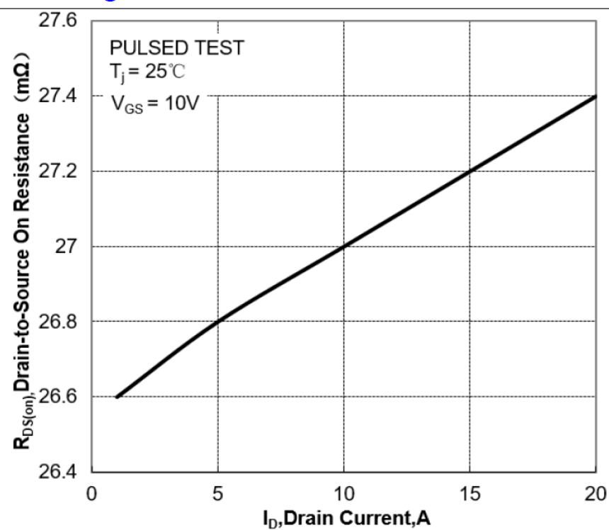
Figure 3 On-Resistance vs. I_D and V_{GS}
