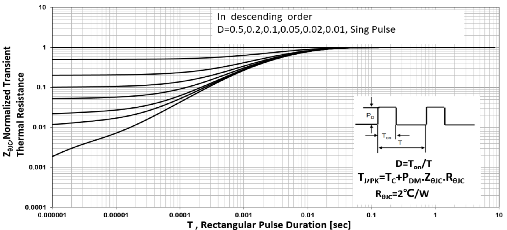
Figure 11 Normalized Maximum Transient Thermal Impedance
