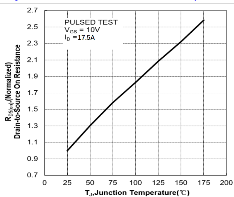
Figure 4 On-Resistance vs. Junction Temperature
