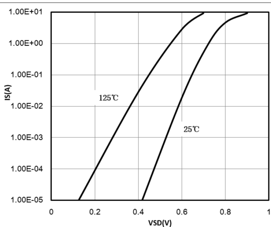
Figure 6 Body Diode Forward Voltage
