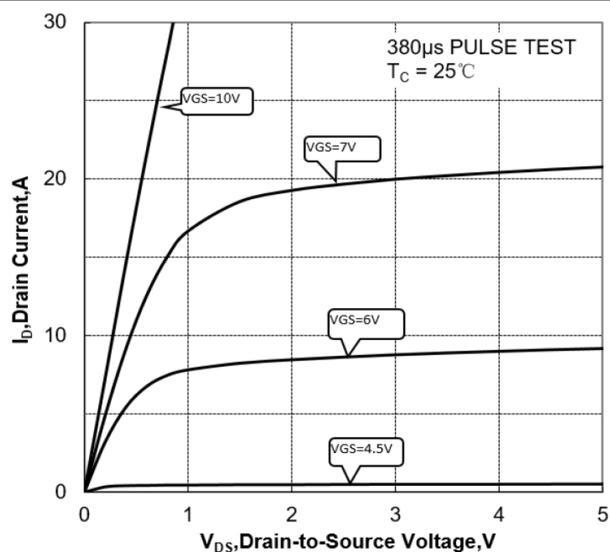
Figure 1 Output Characteristics
