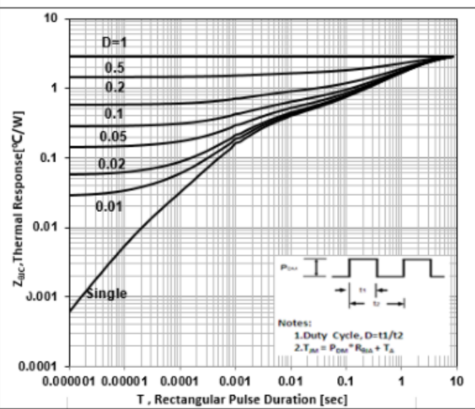
Figure 3b Max Thermal Impedance (FullPAK)
