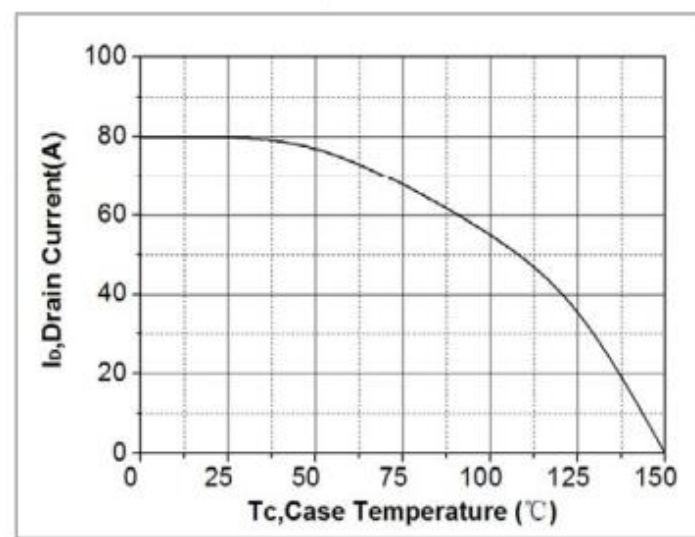
Fig. 10. Maximum drain current vs. case temperature
