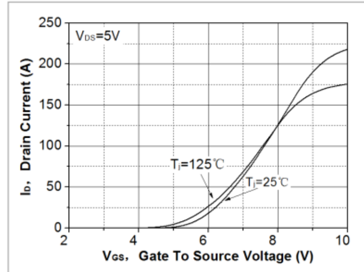
Fig. 2. Transfer Characteristics
