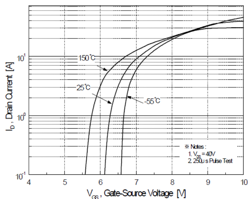
Figure 2. Transfer Characteristics
