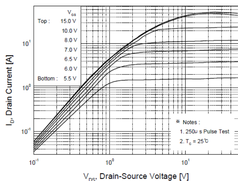
Figure 1. On-Region Characteristics
