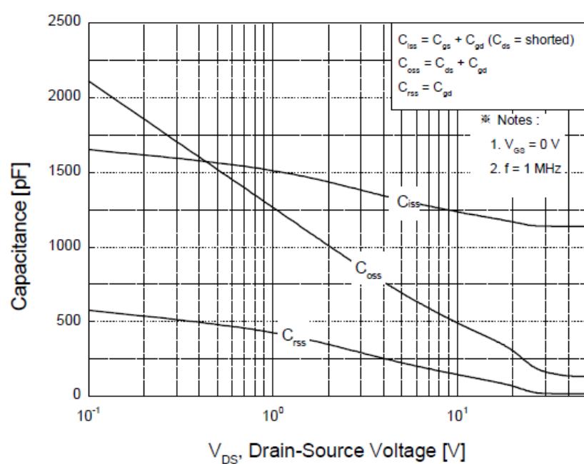
Figure 5. Capacitance Characteristics
