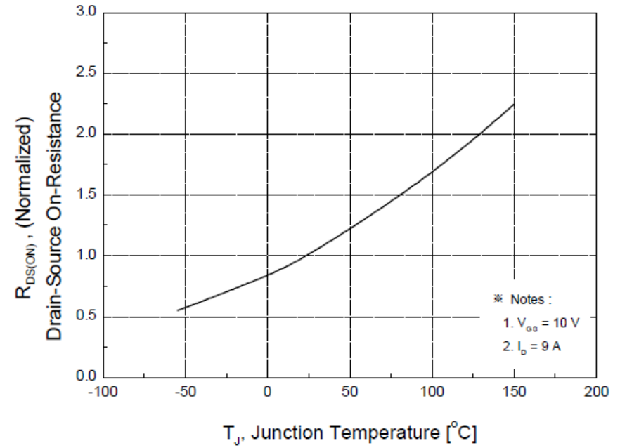
Figure 8. On-Resistance Variation
