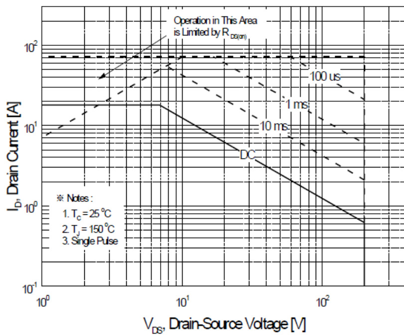
Figure 9. Maximum Safe Operating Area
