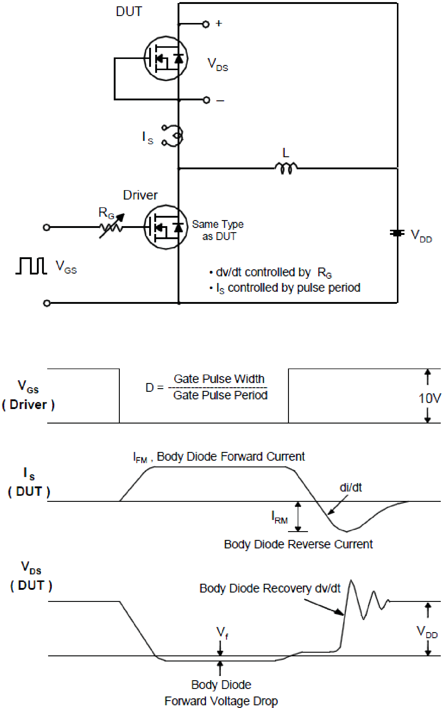
Fig 15. Peak Diode Recovery dv/dt Test Circuit & Waveforms
