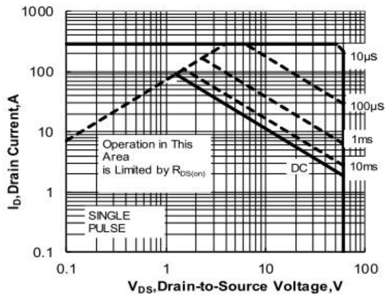
Figure 9. Maximum Safe Operating
