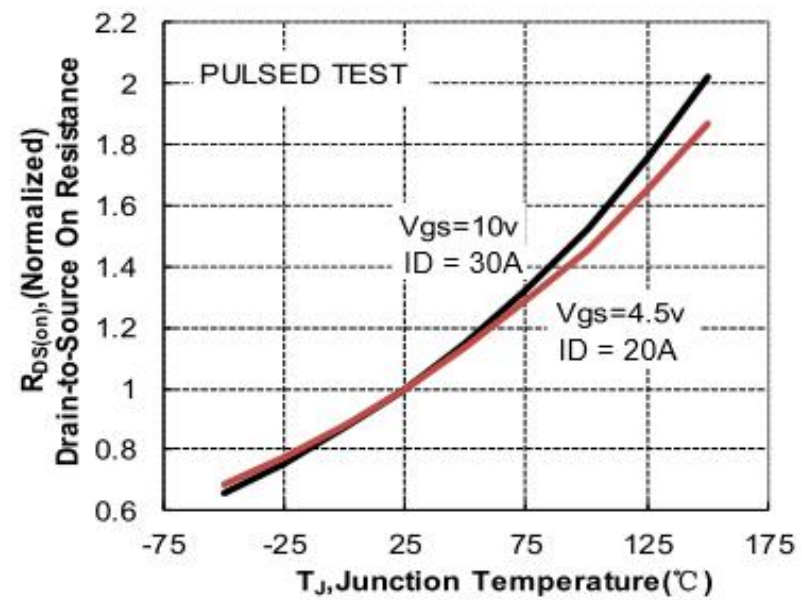
Figure 8. Normalized On Resistance vs Junction Temperature
