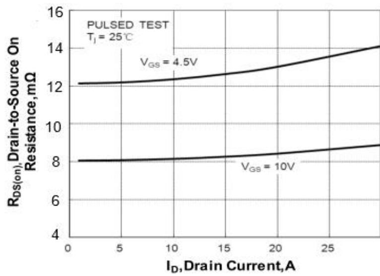
Figure 3. Drain-to-Source On Resistance vs Drain Current
