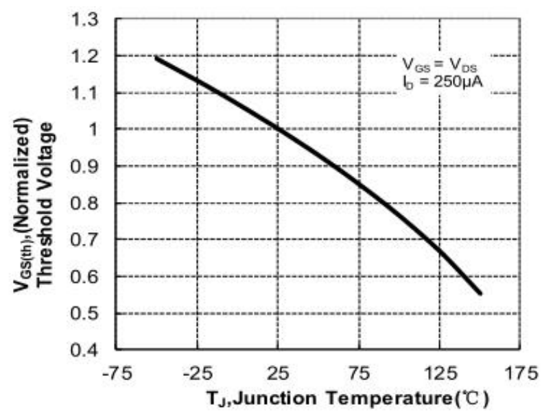
Figure 10. Normalized Threshold Voltage vs Junction Temperature
