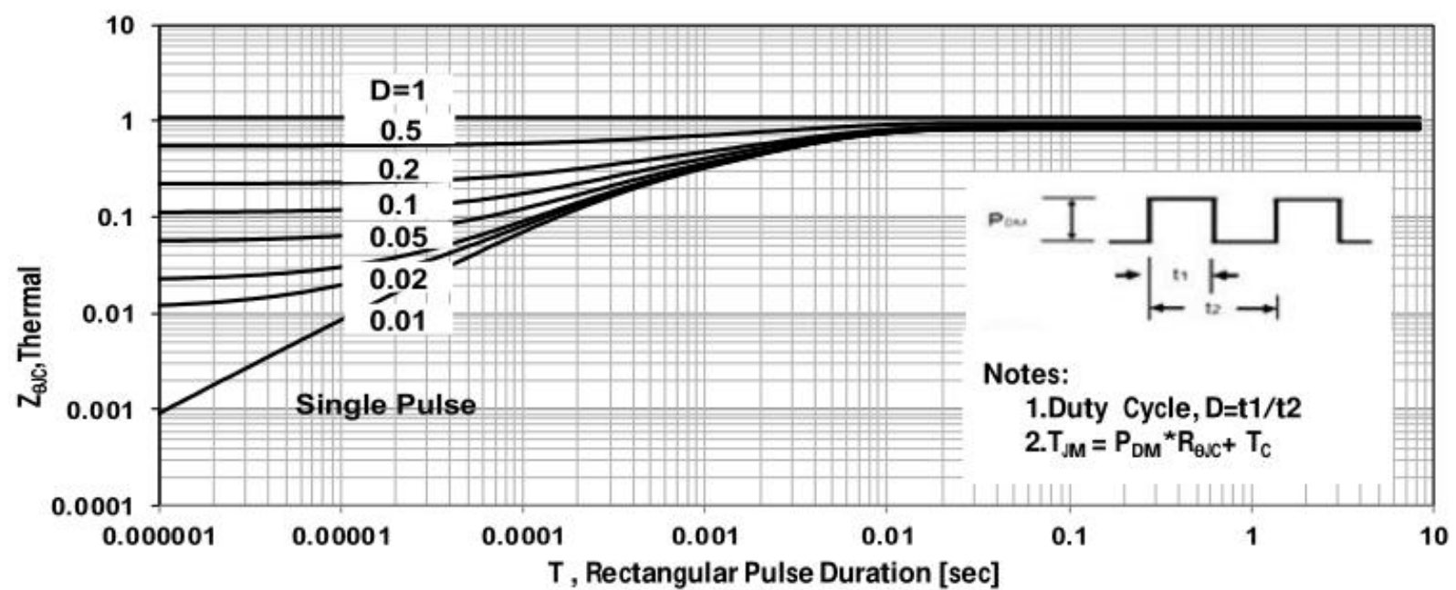
Figure 11. Maximum Effective Transient Thermal Impedance, Junction-to-Case
