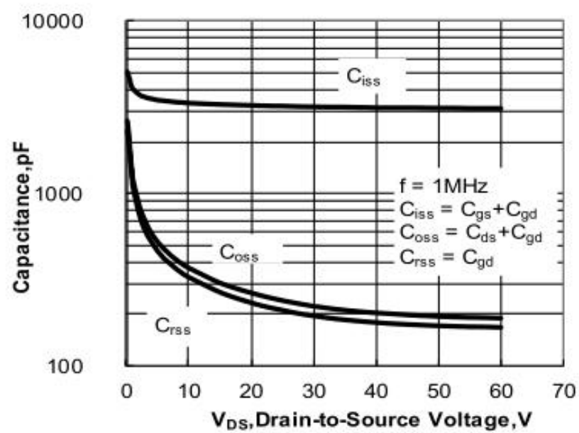
Figure 5. Capacitance Characteristics
