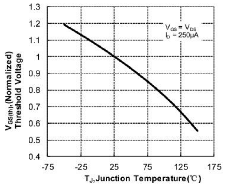
Figure 13. Normalized Threshold Voltage vs Junction Temperature
