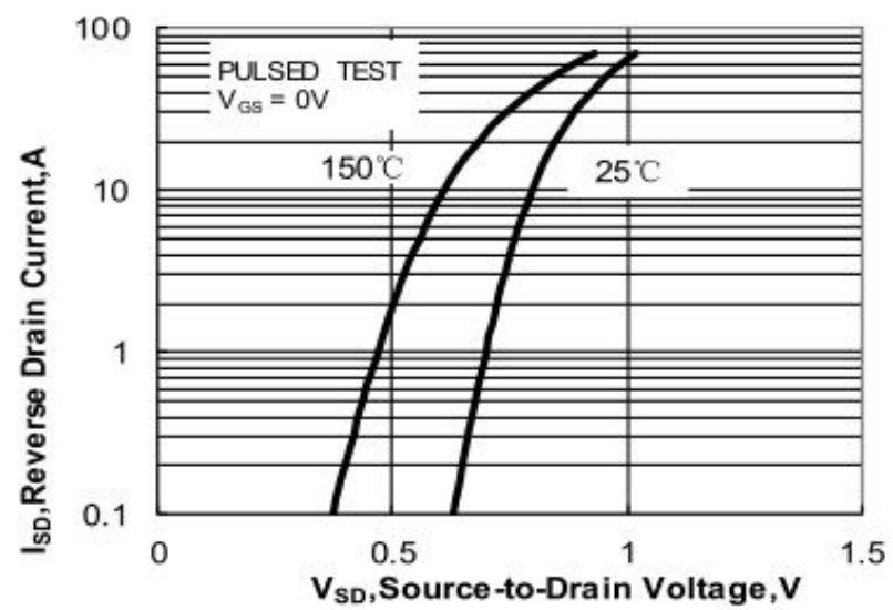
Figure 4. Typical Body Diode Transfer Characteristics
