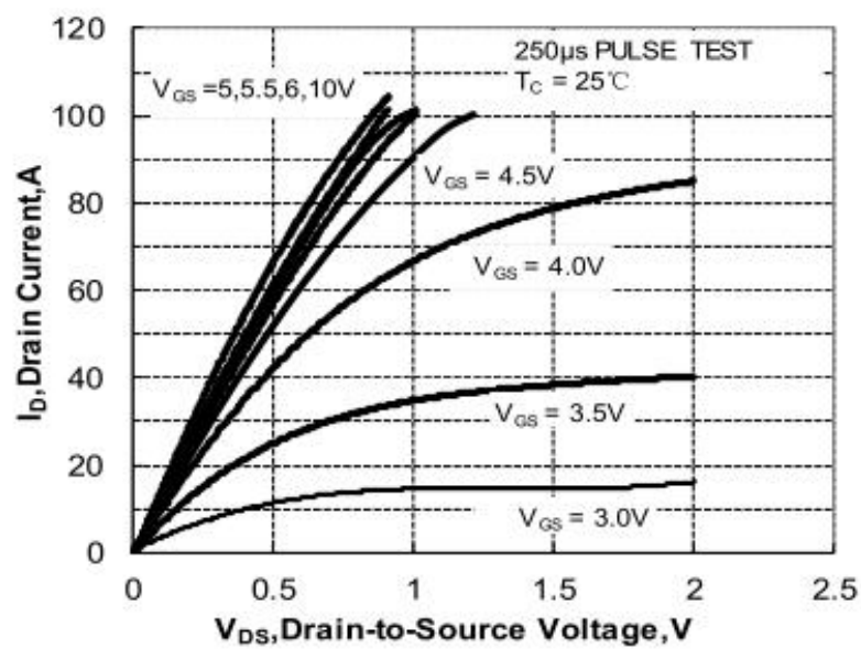
Figure 1. Output Characteristics
