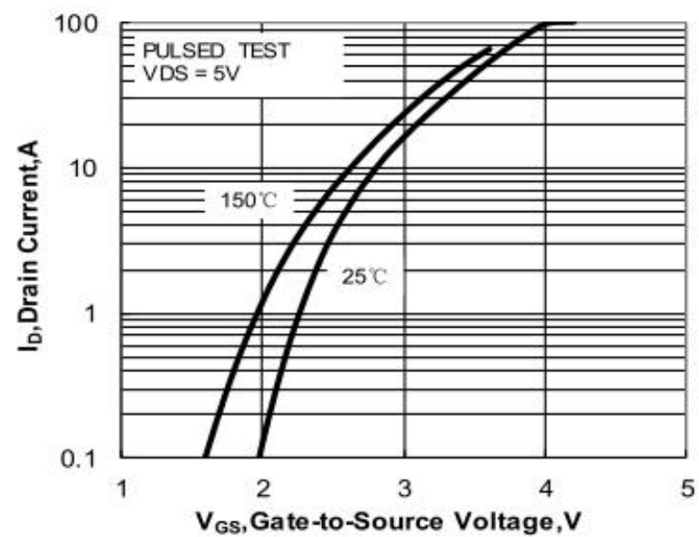
Figure 2. Transfer Characteristics
