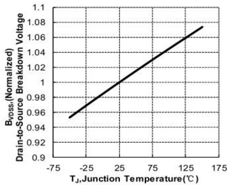
Figure 7. Normalized Breakdown Voltage vs Junction Temperature
