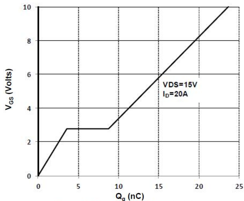
Figure 7: Gate-Charge Characteristics
