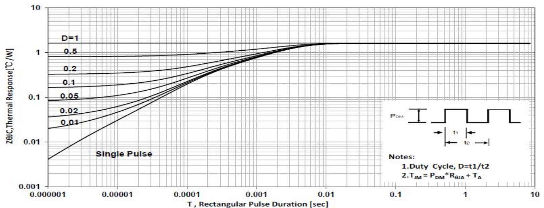
Figure 11: Normalized Maximum Transient Thermal Impedance
