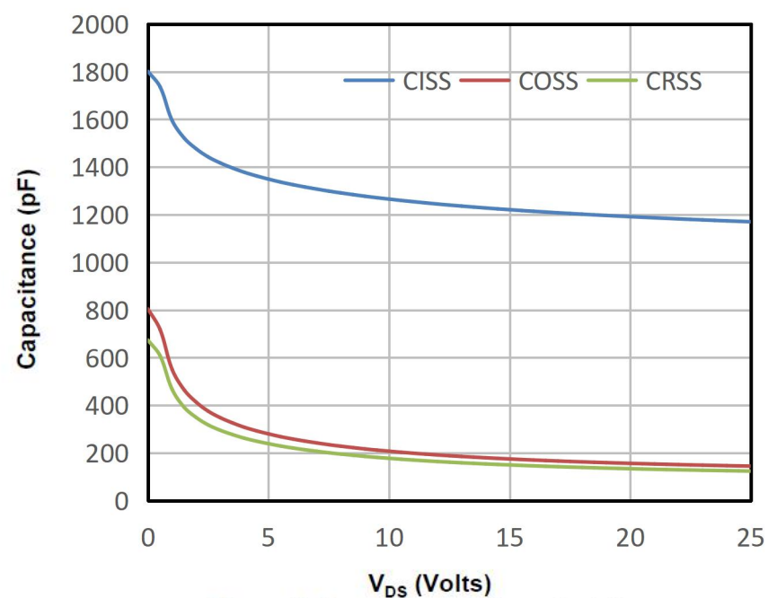
Figure 8: Capacitance Characteristics
