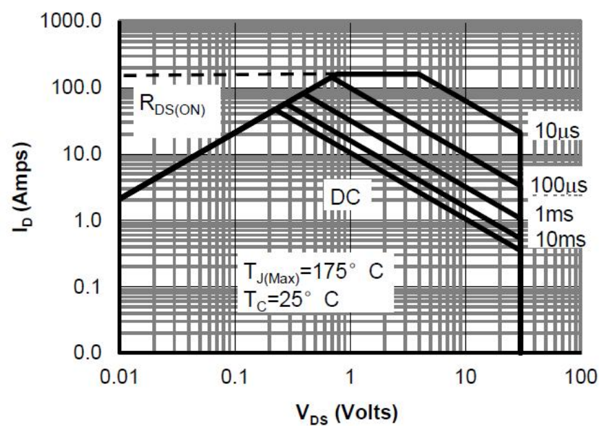
Figure 9: Maximum Forward Biased Safe Operating Area
