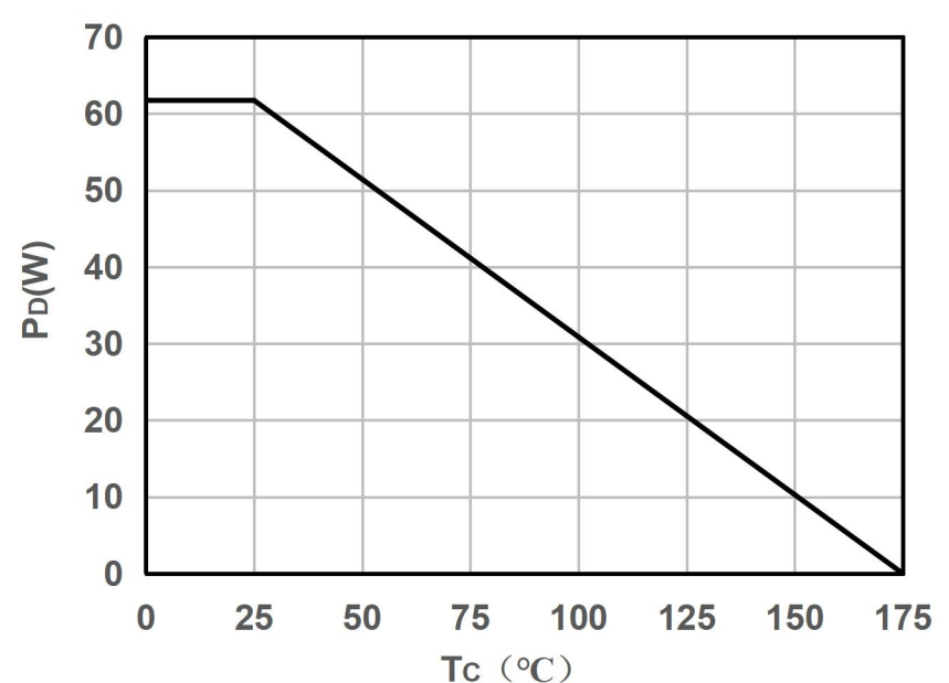
Figure 10: Maximum Power Dissipation vs Case Temperature
