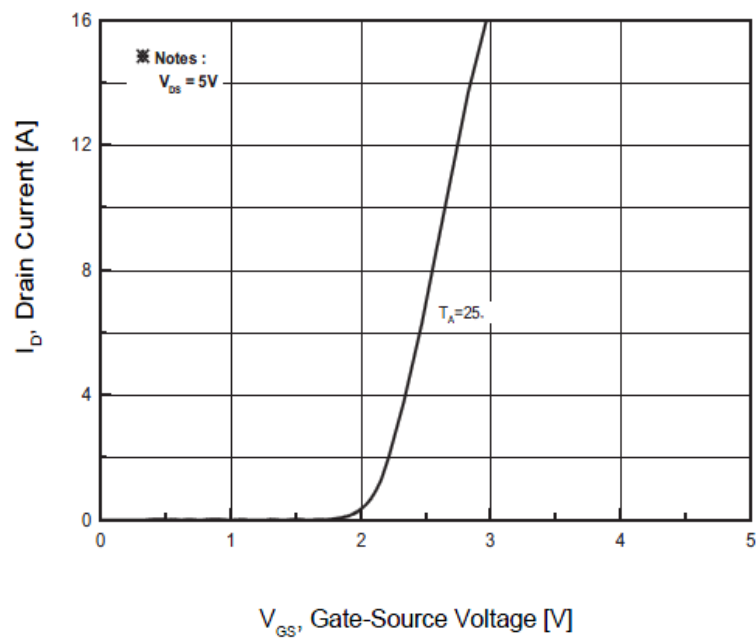
Fig.5 Transfer Characteristics
