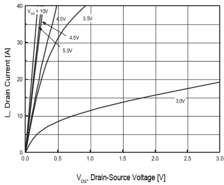
Fig.1 On-Region Characteristics
