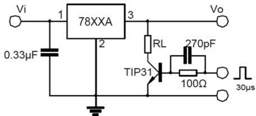
FIG.3 LOAD REGULATION
