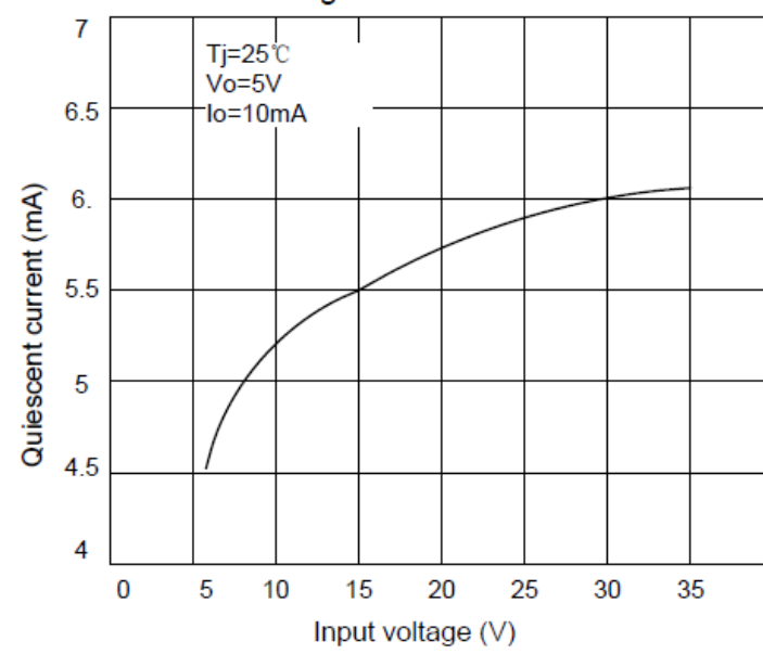
Fig.17 Quiescent current
