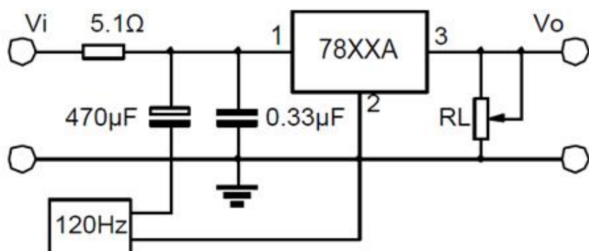
FIG.4 RIPPLE REJECTION
