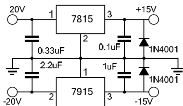
Fig.11 Split power supply ($\pm 15\text{V}, 1\text{A}$)
