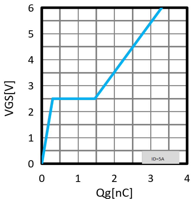
Fig.9:Gate Charge
