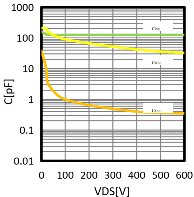
Fig.4: Typical Capacitance
