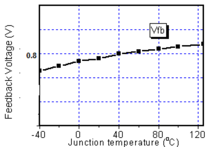
Figure 5. Vfb vs. Temperature
