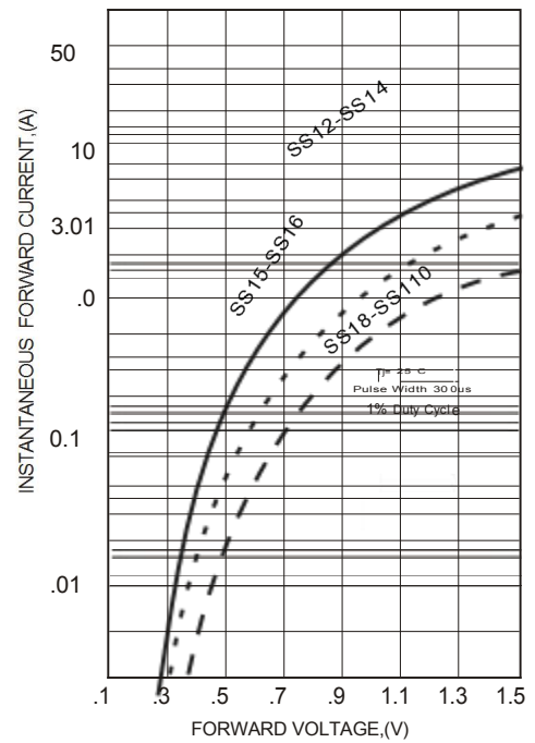
FIG.2-TYPICAL FORWARD CHARACTERISTICS
