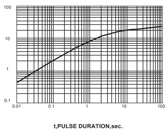
FIG. 6-TYPICAL TRANSIENT THERMALIMPEDANCE
