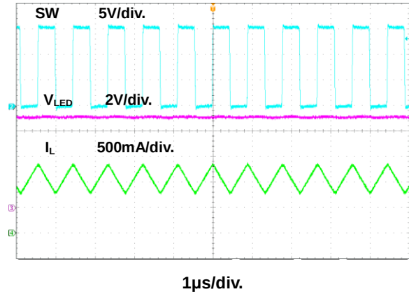
Figure 7. Switching Waveform
