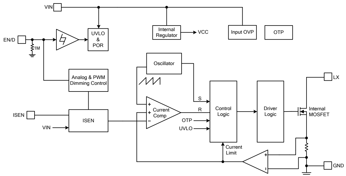
Figure 5. Block Diagram of FR9708
