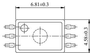
SOP6-P
