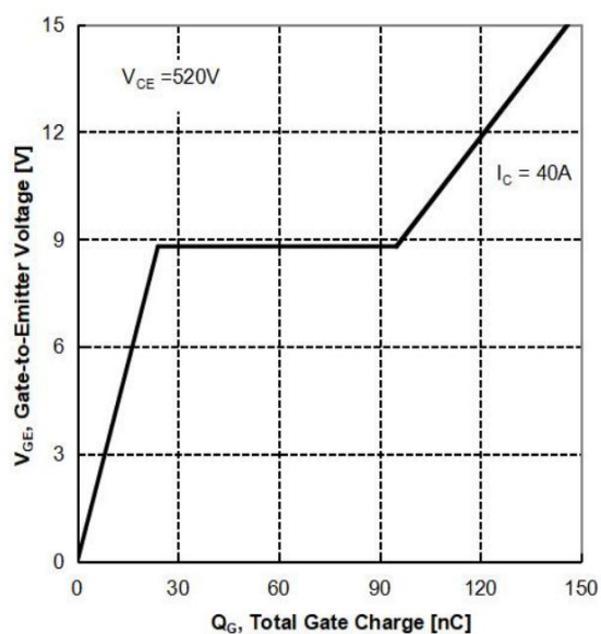
Figure 17: Typical Gate Charge
