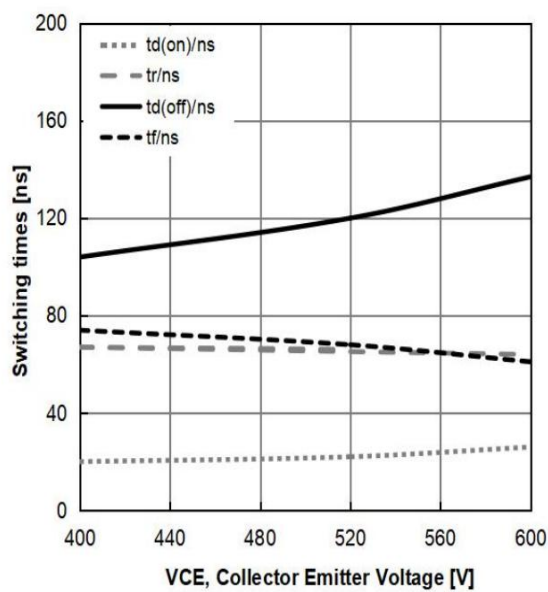
Figure 15: Typical Switching Times vs. VCE ( T_J=25^{\circ}\text{C} , V_{GE}=15/0\text{V} , I_C=40\text{A} )
