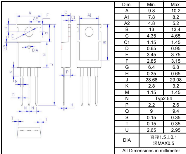
TO-220C
