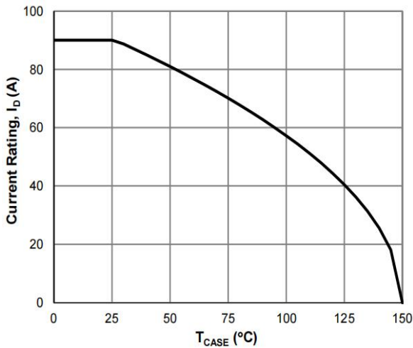
Figure 7: Current De-rating
