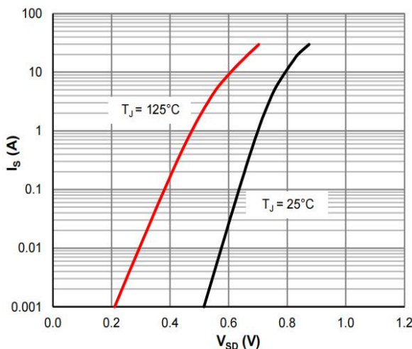
Figure 5: Body-Diode Characteristics
