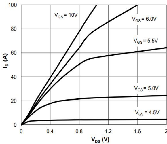
Figure 1: Saturation Characteristics
