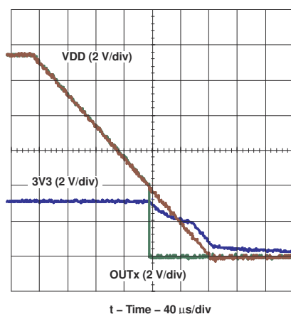
图 8-16. Shut Down Behavior at V_{DD} = 12\text{ V} (Input Tied to 3V3)
