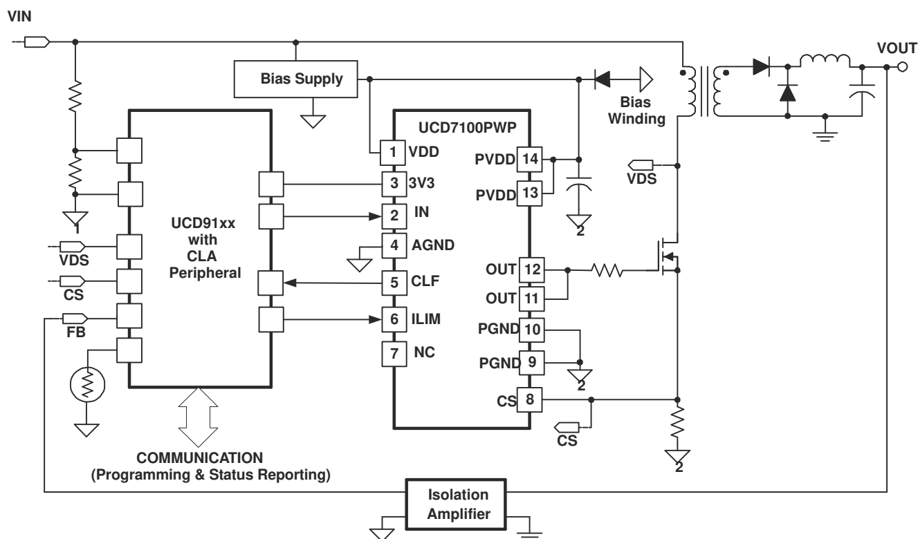
图 12-1. Isolated Forward Converter
