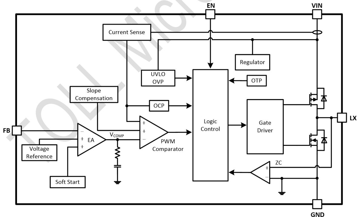
Figure 2. TMI3113B Block Diagram
